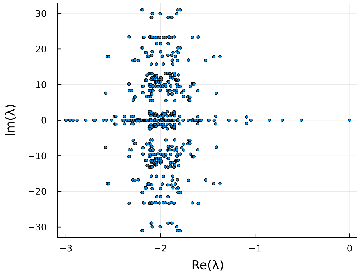
Full Diagonalization
