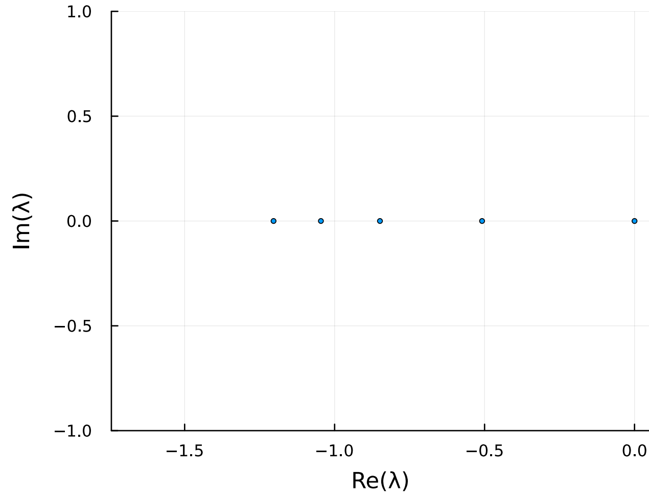
SCI Approximation
