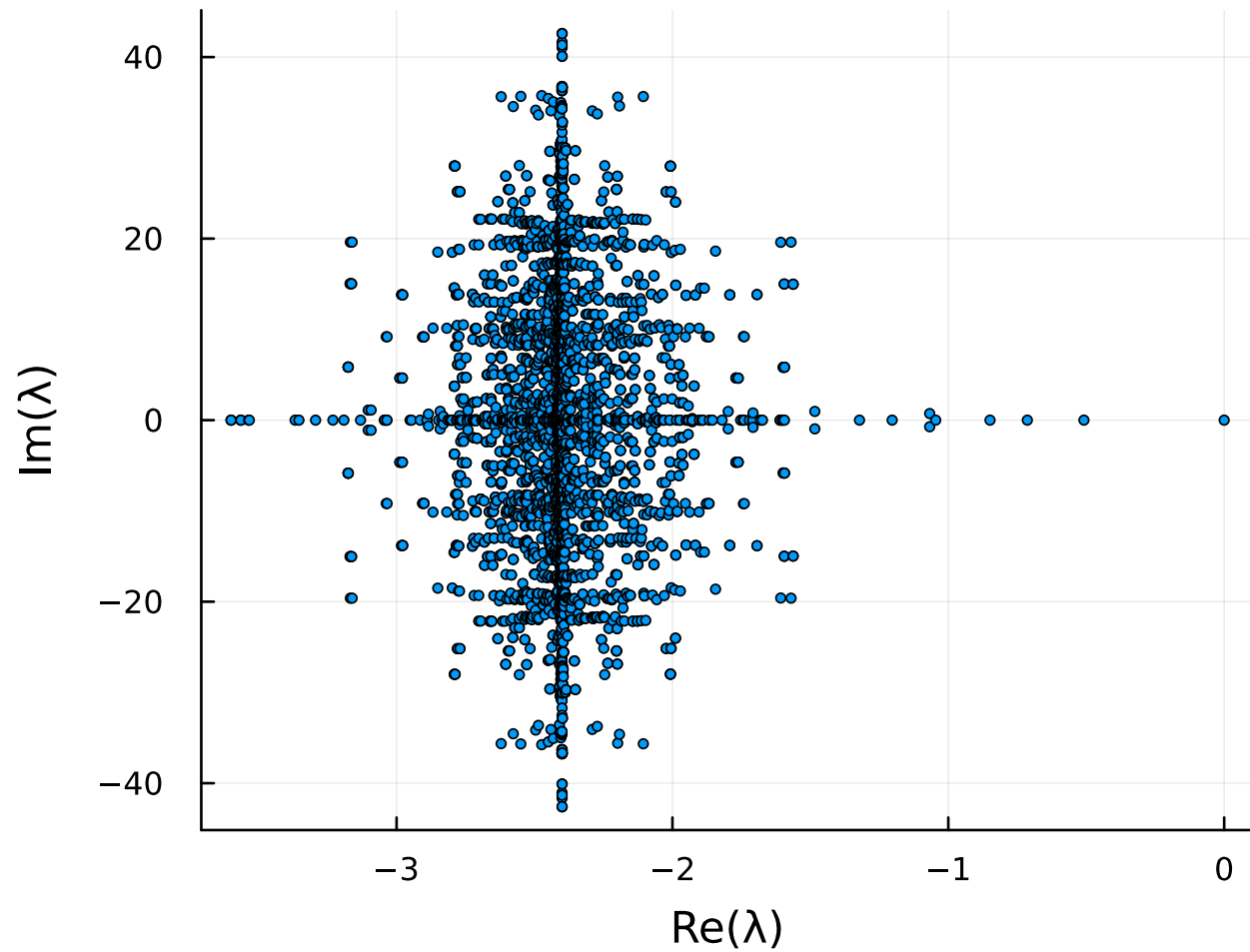
Full Diagonalization
