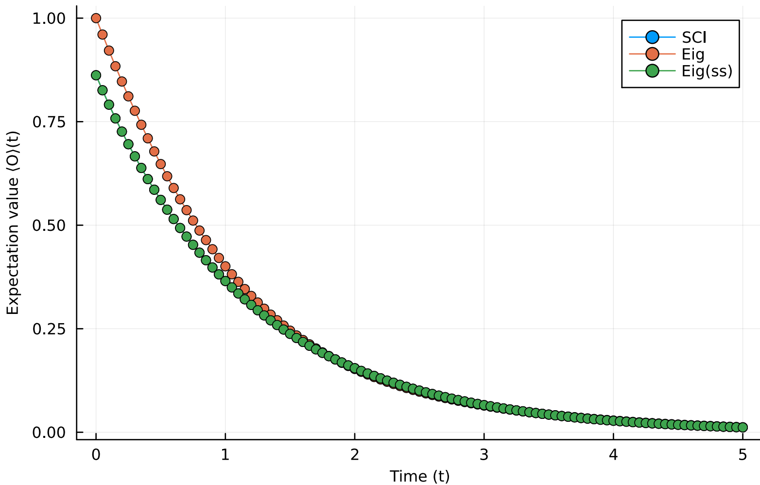
Expectation value of ZZI using SCI(R = 4) and Eigendecomposition of L for N=3
