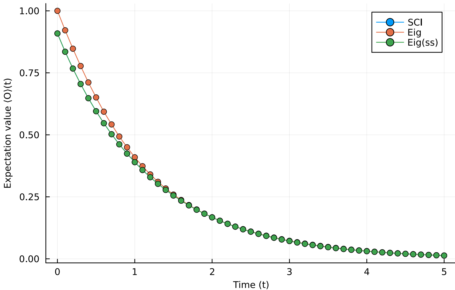
Expectation value of ZZII using SCI(R = 4) and Eigendecomposition of L for N=4
