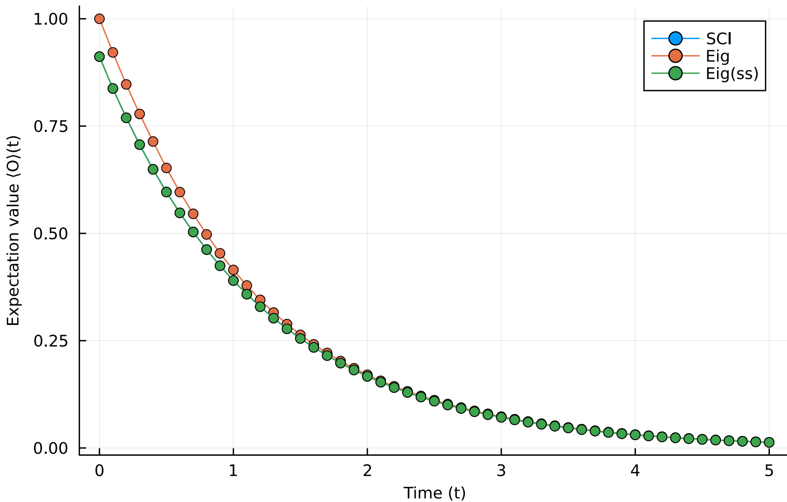
Expectation value of ZZIII using SCI(R = 6) and Eigendecomposition of L for N=5
