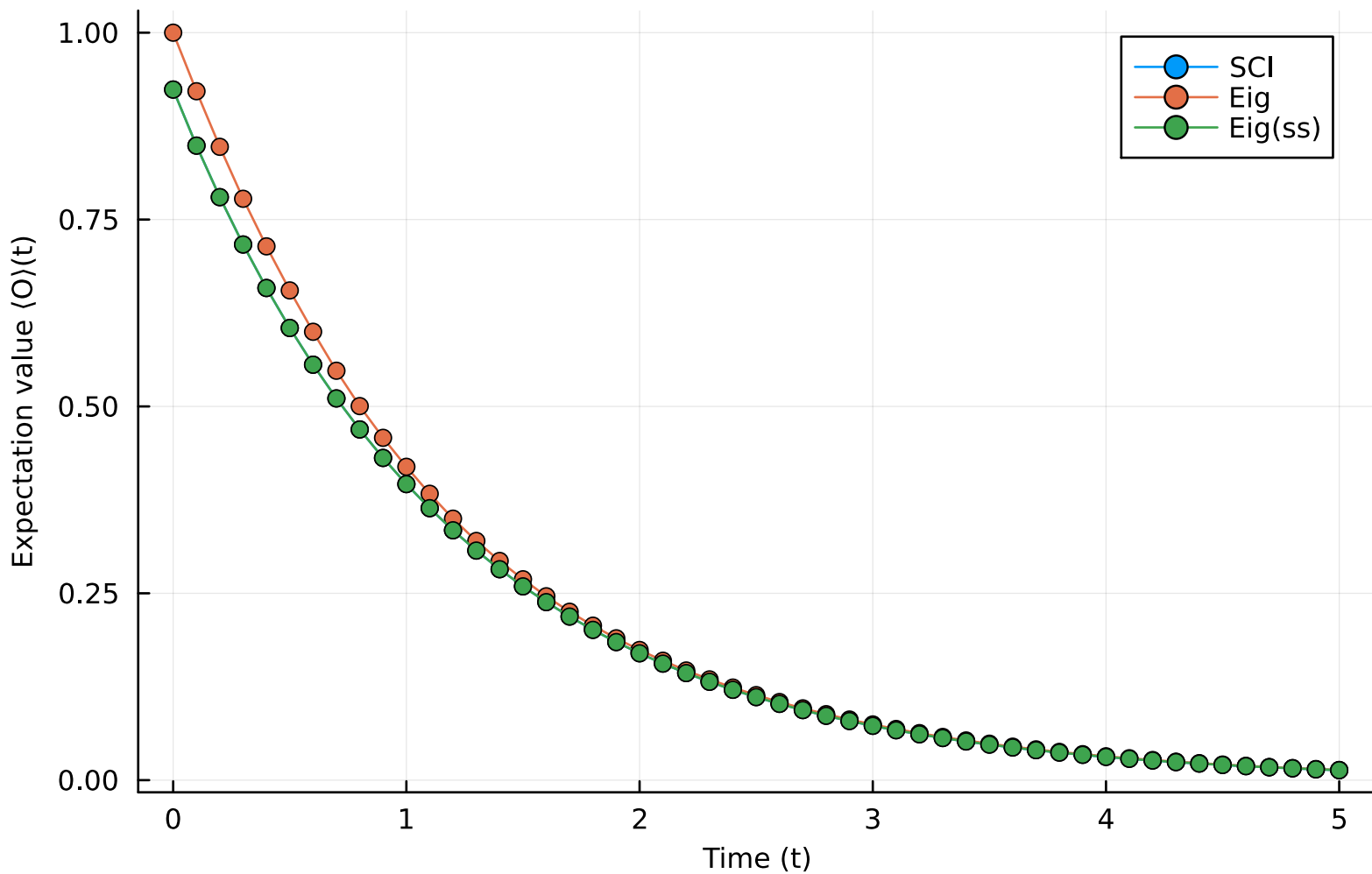
Expectation value of ZZIIII using SCI(R = 6) and Eigendecomposition of L for N=6
