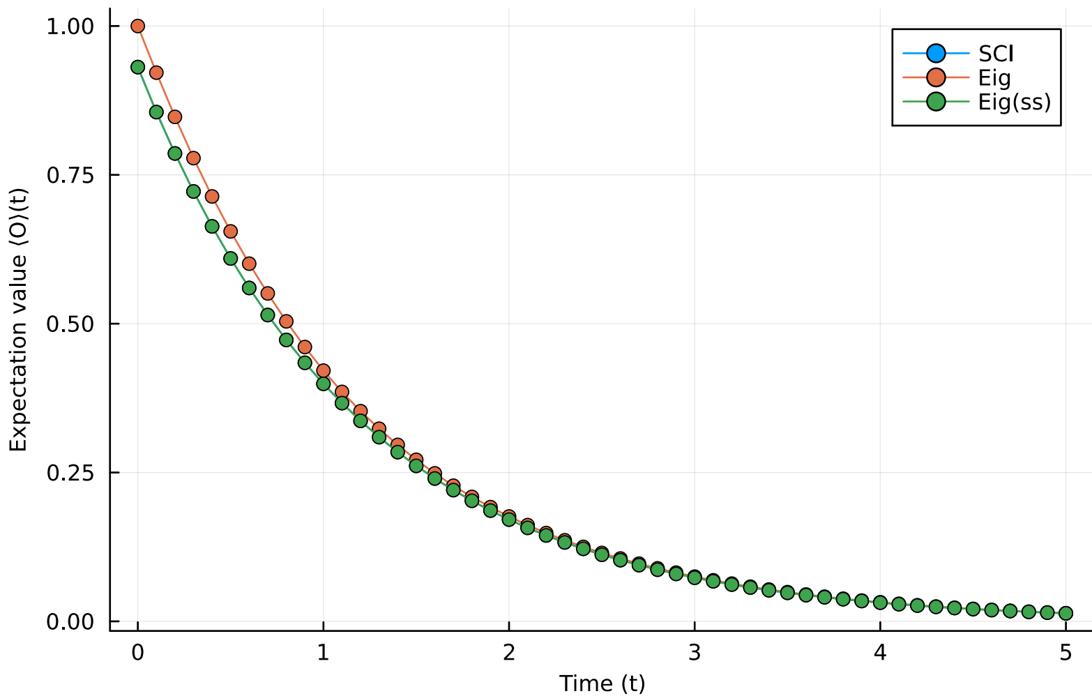
Expectation value of ZZIIII using SCI(R = 6) and Eigendecomposition of L for N=7
