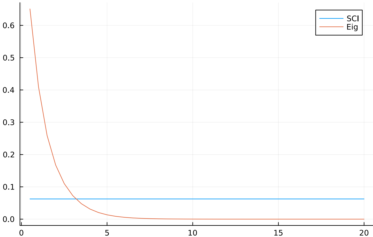
Expectation value of Z_1 using SCI( R = 1 ) and Eigendecomposition of L
