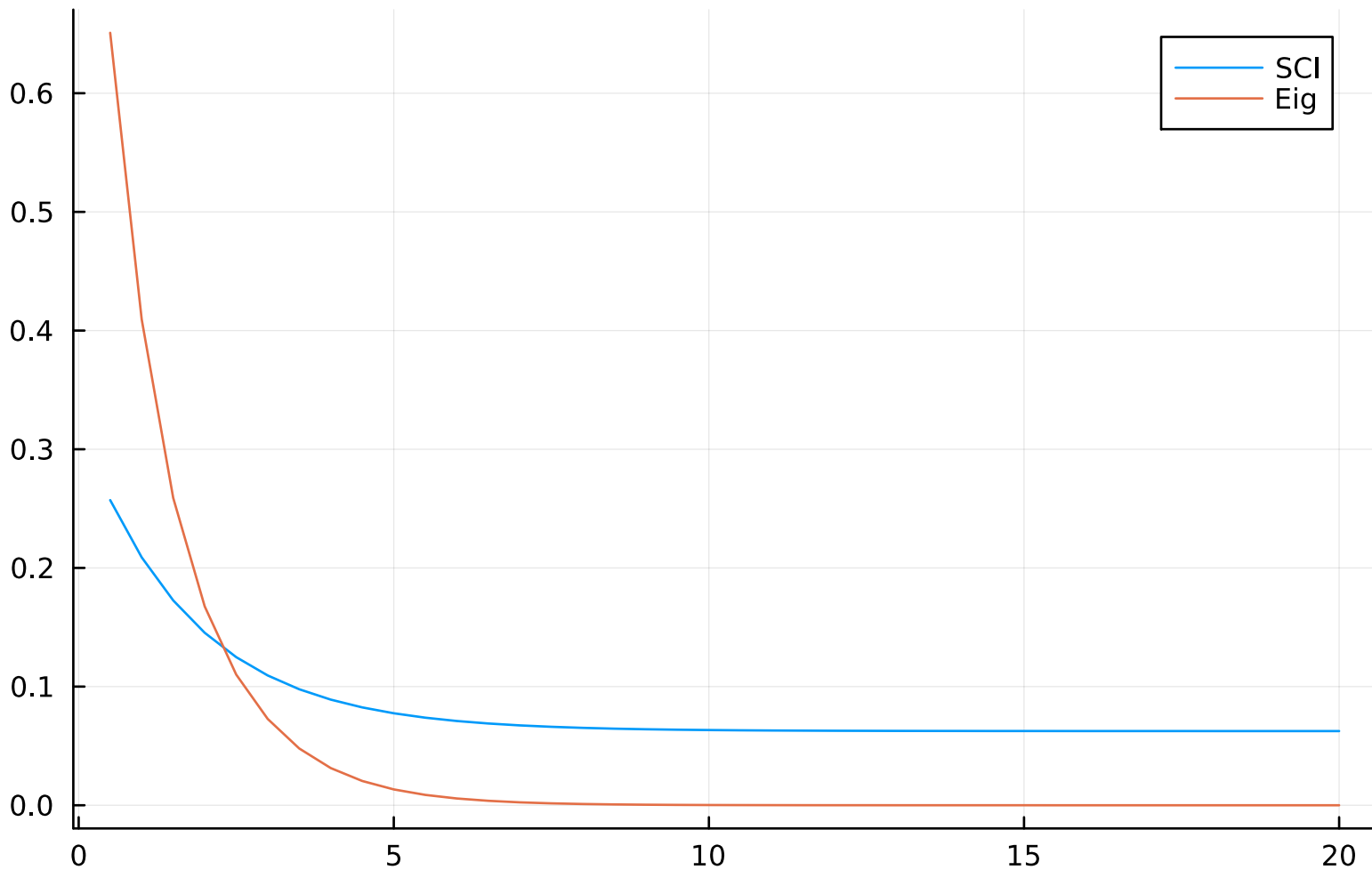
Expectation value of Z_1 using SCI( R = 2 ) and Eigendecomposition of L
