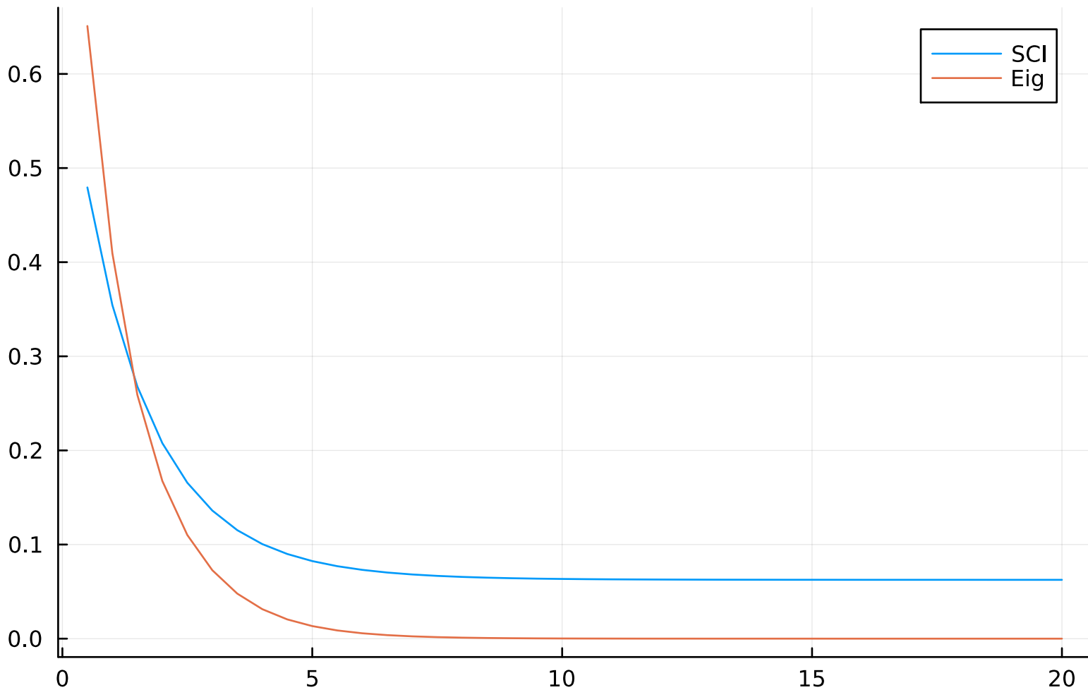
Expectation value of Z_1 using SCI( R = 3 ) and Eigendecomposition of L
