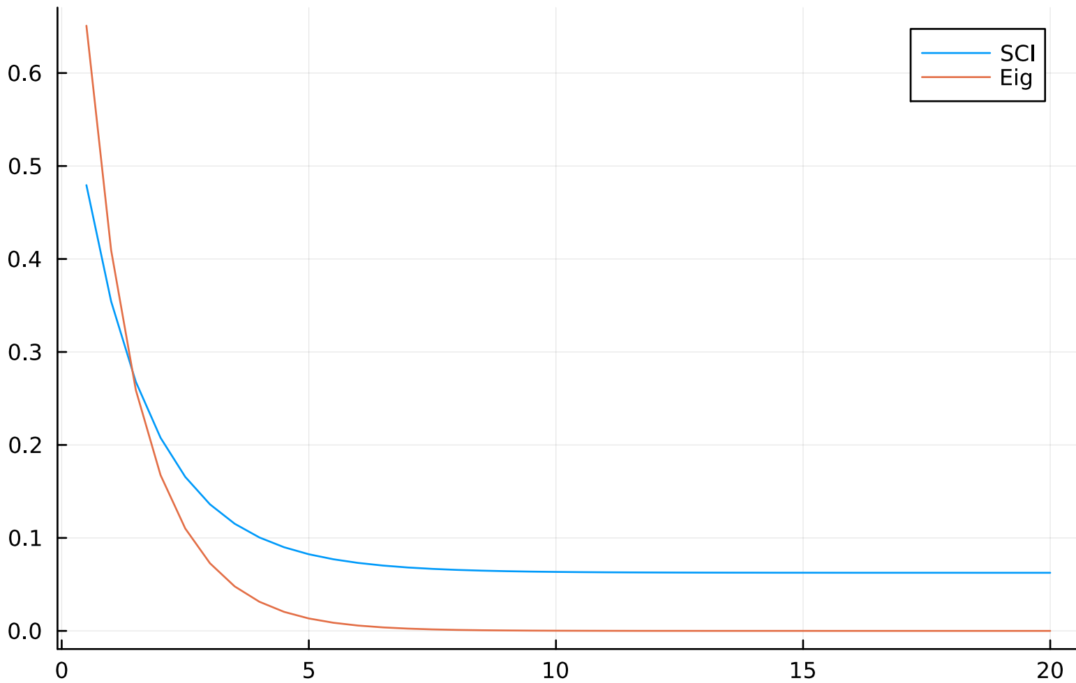
Expectation value of Z_1 using SCI( R = 7 ) and Eigendecomposition of L
