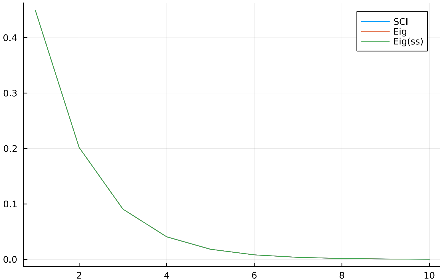
Expectation value of ZZ using SCI(R = 3) and Eigendecomposition of L for N=2
