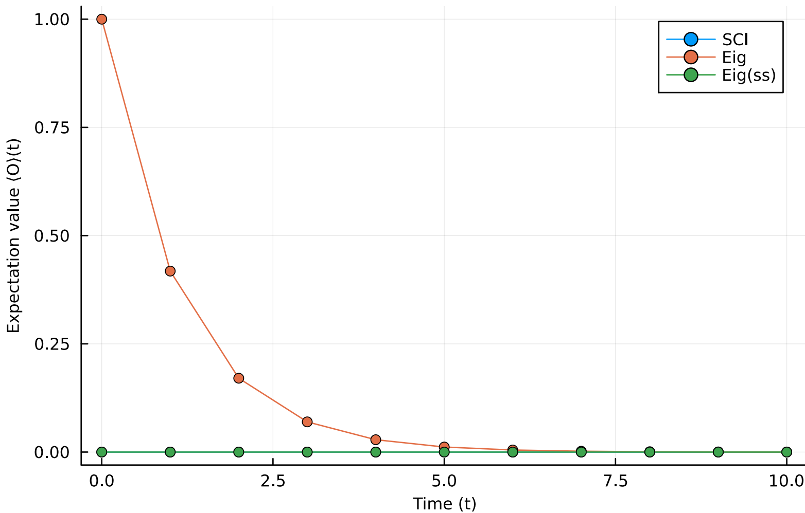
Expectation value of ZZI using SCI(R = 2) and Eigendecomposition of L for N=3
