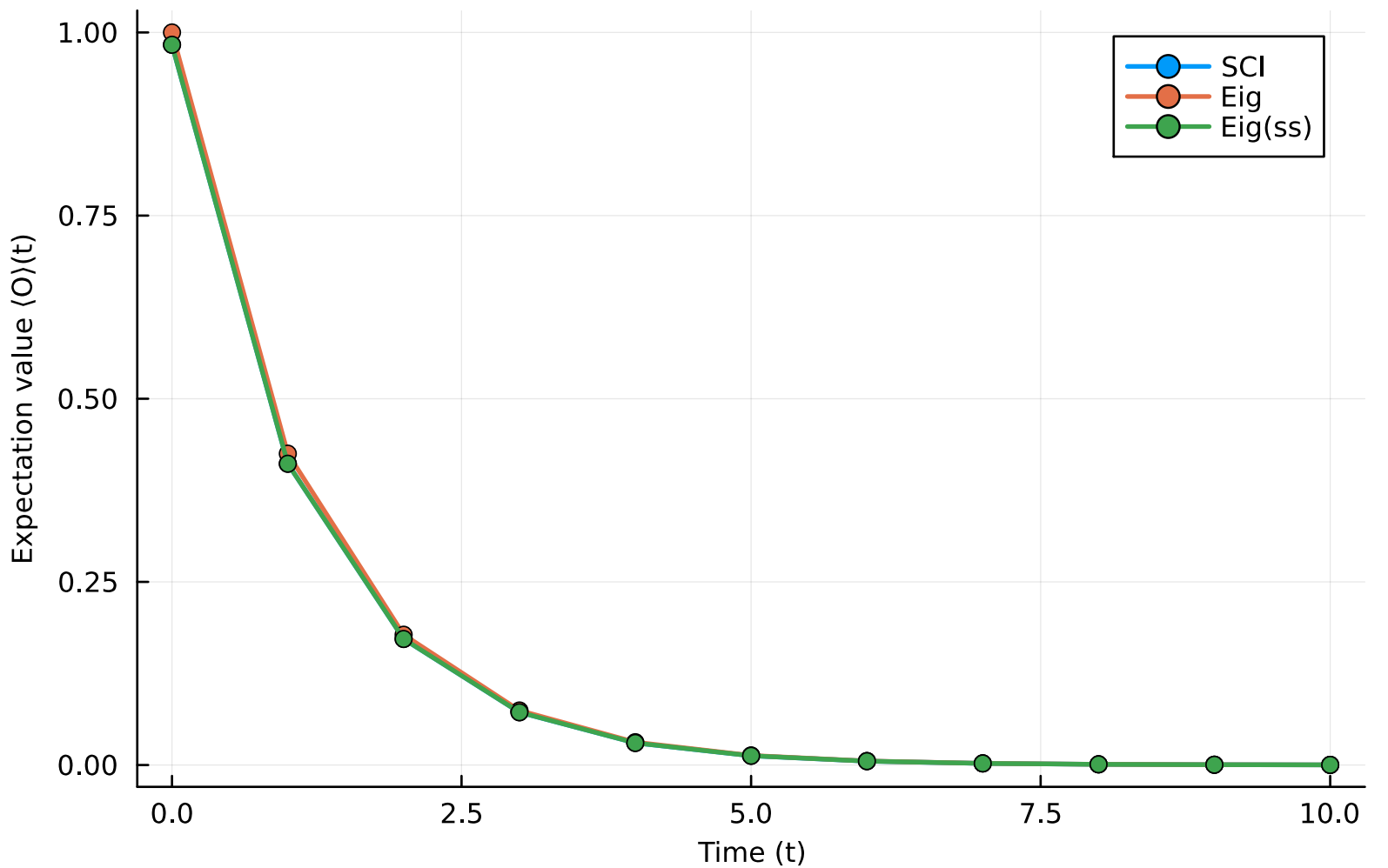
Expectation value of ZZIII using SCI(R = 3) and Eigendecomposition of L for N=5
