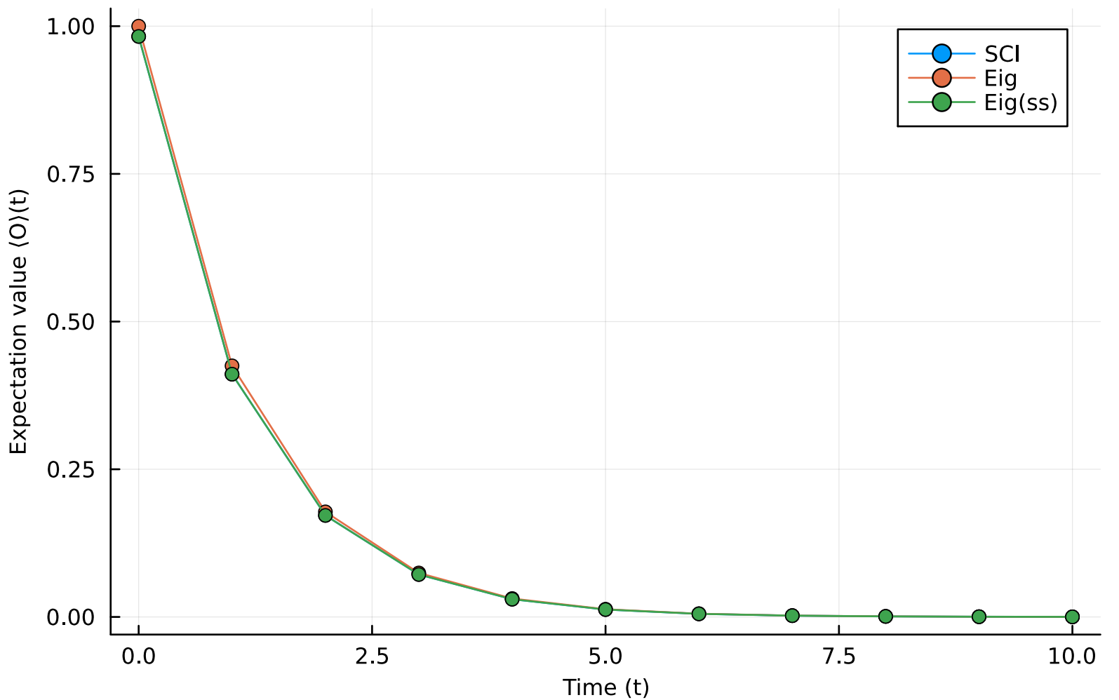
Expectation value of ZZIII using SCI(R = 4) and Eigendecomposition of L for N=5
