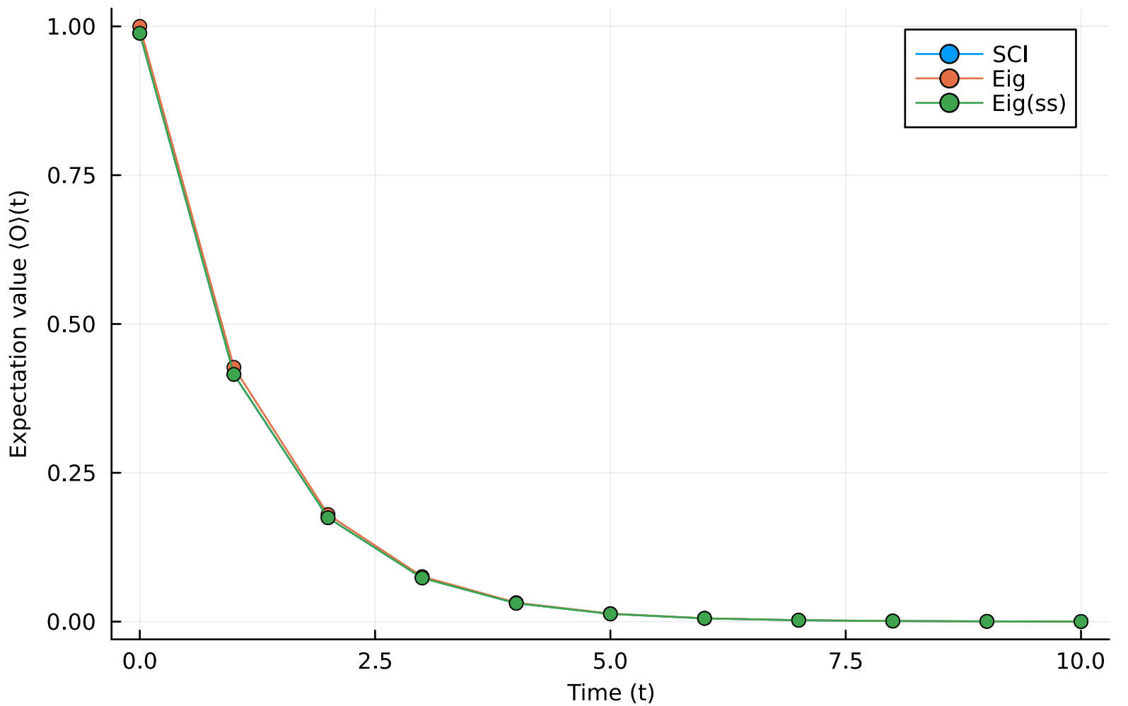
Expectation value of ZZIIII using SCI(R = 4) and Eigendecomposition of L for N=6
