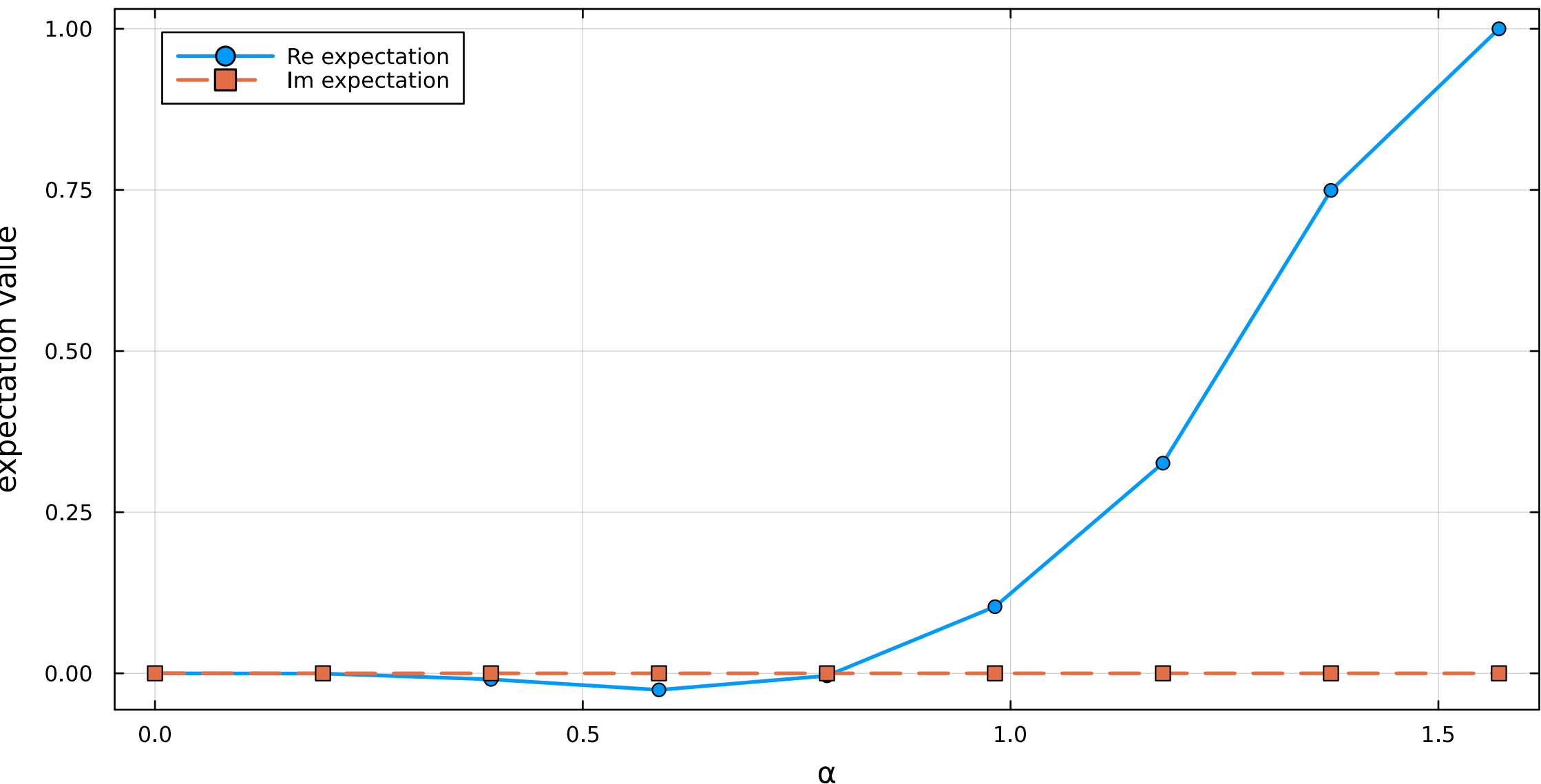
Eagle processor observable
