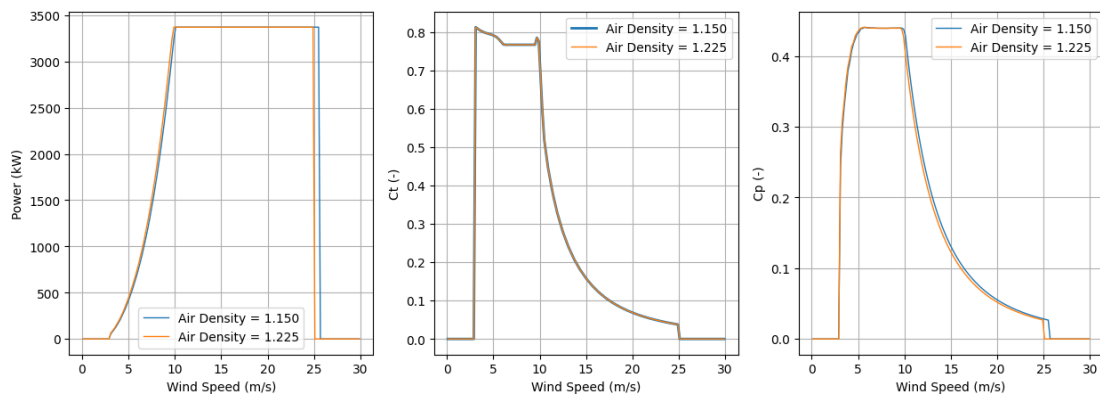
Figure 2: Turbine characteristic plots for power, C_p , and C_t (from FLORIS and not from CSV).
