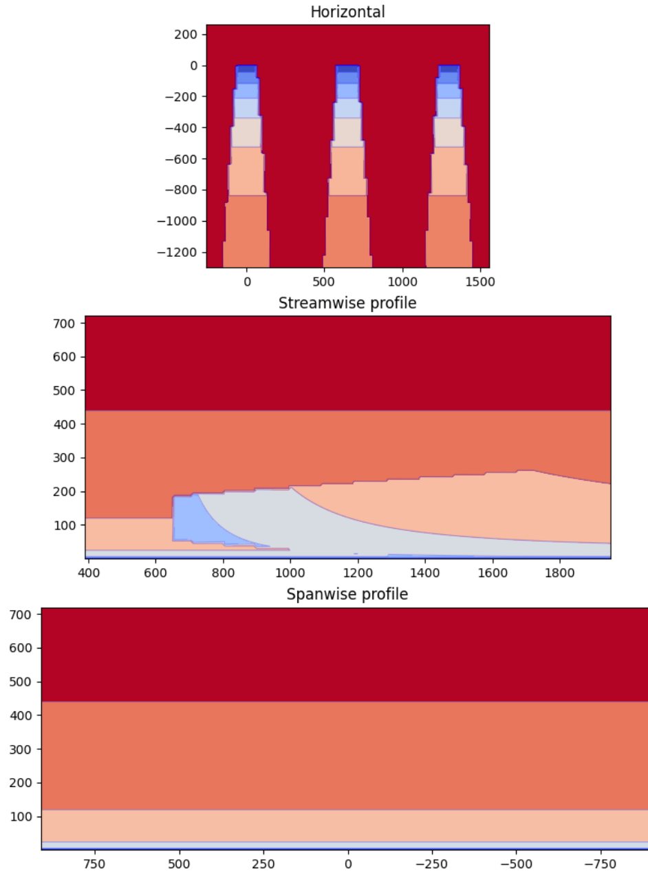
Figure 4: Horizontal, streamwise, and cross-plane flow visualization for the 0^\circ case.
