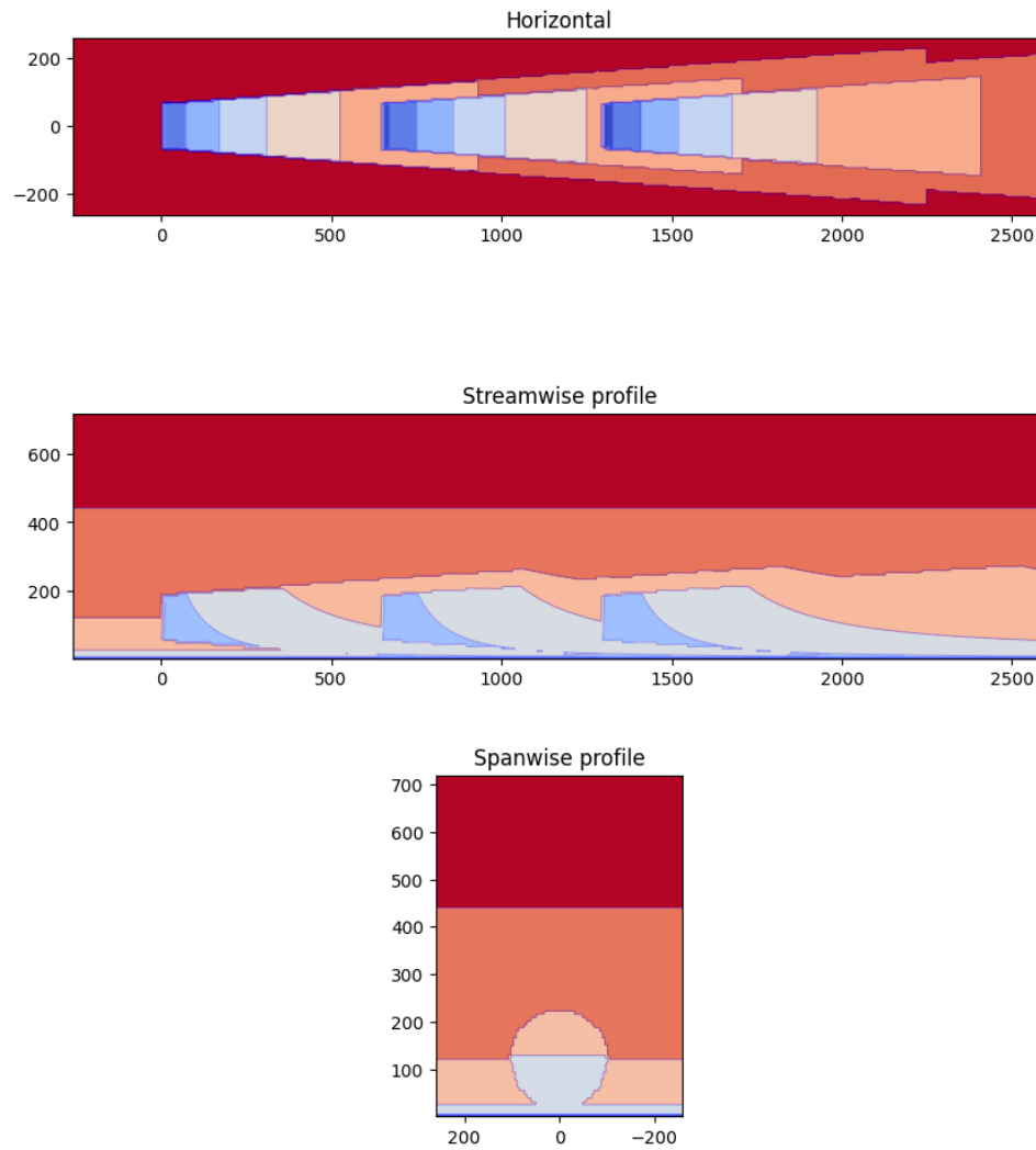
Figure 5: Horizontal, streamwise, and cross-plane flow visualization for the 270° case.
