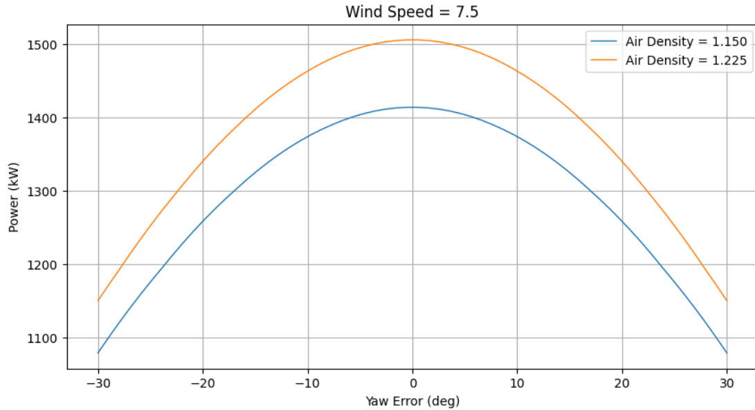
Figure 3: Power variation with yaw error in the range [-30^\circ, 30^\circ] .
