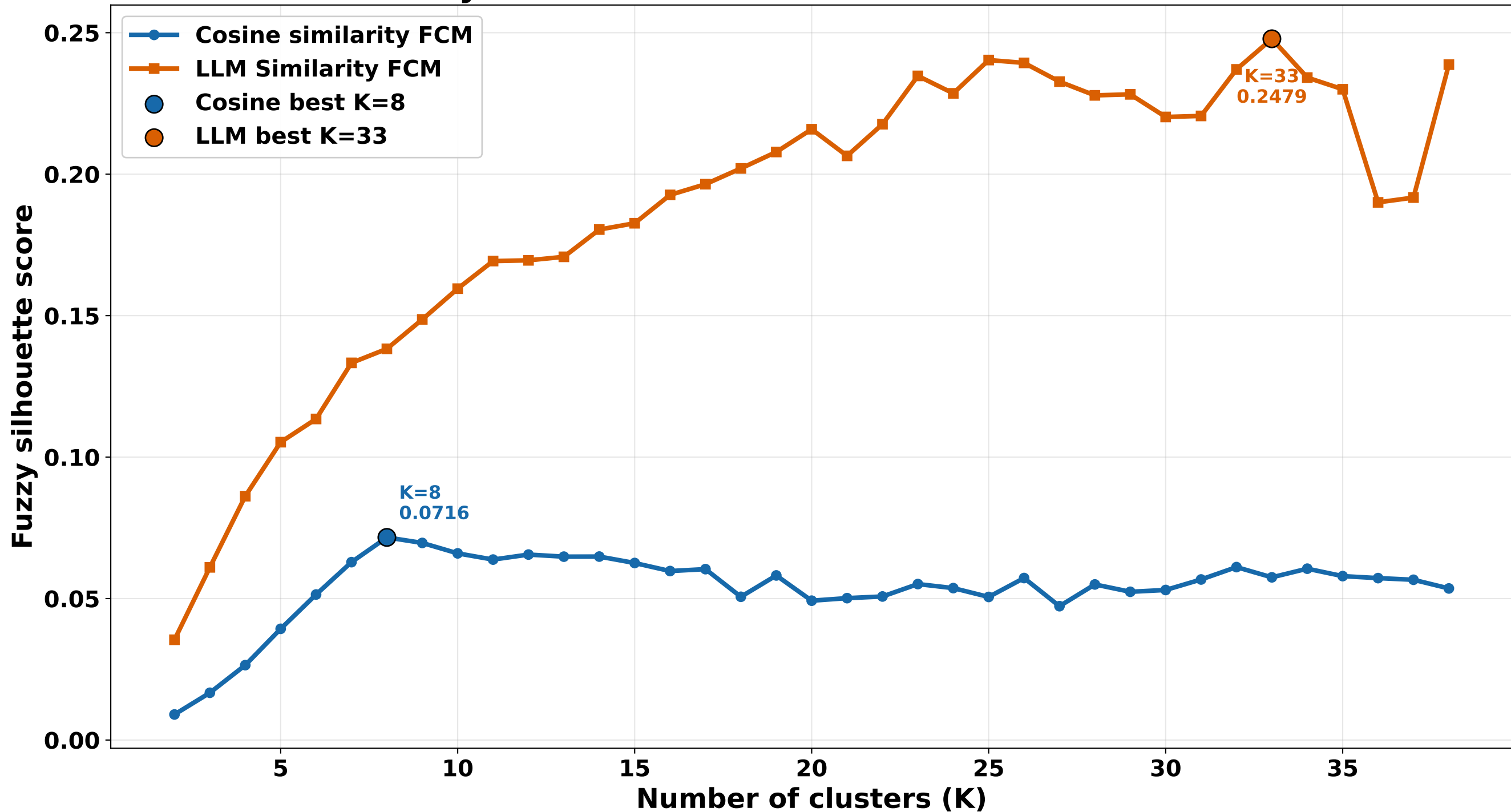
Fuzzy Silhouette Score vs. Number of Clusters
