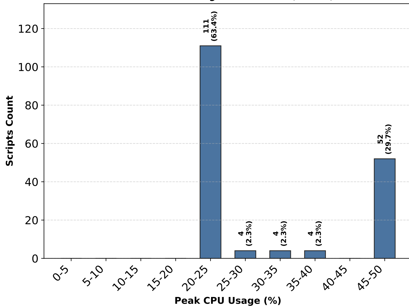
A. Peak CPU Usage Distribution (n=175)
