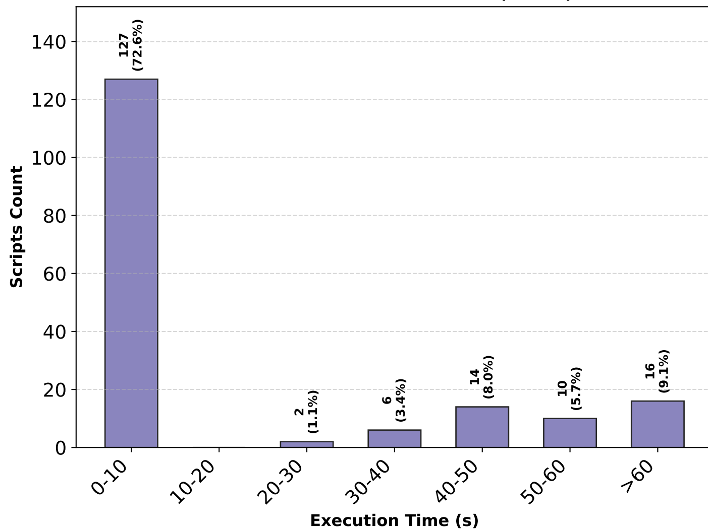
C. Execution Time Distribution (n=175)
