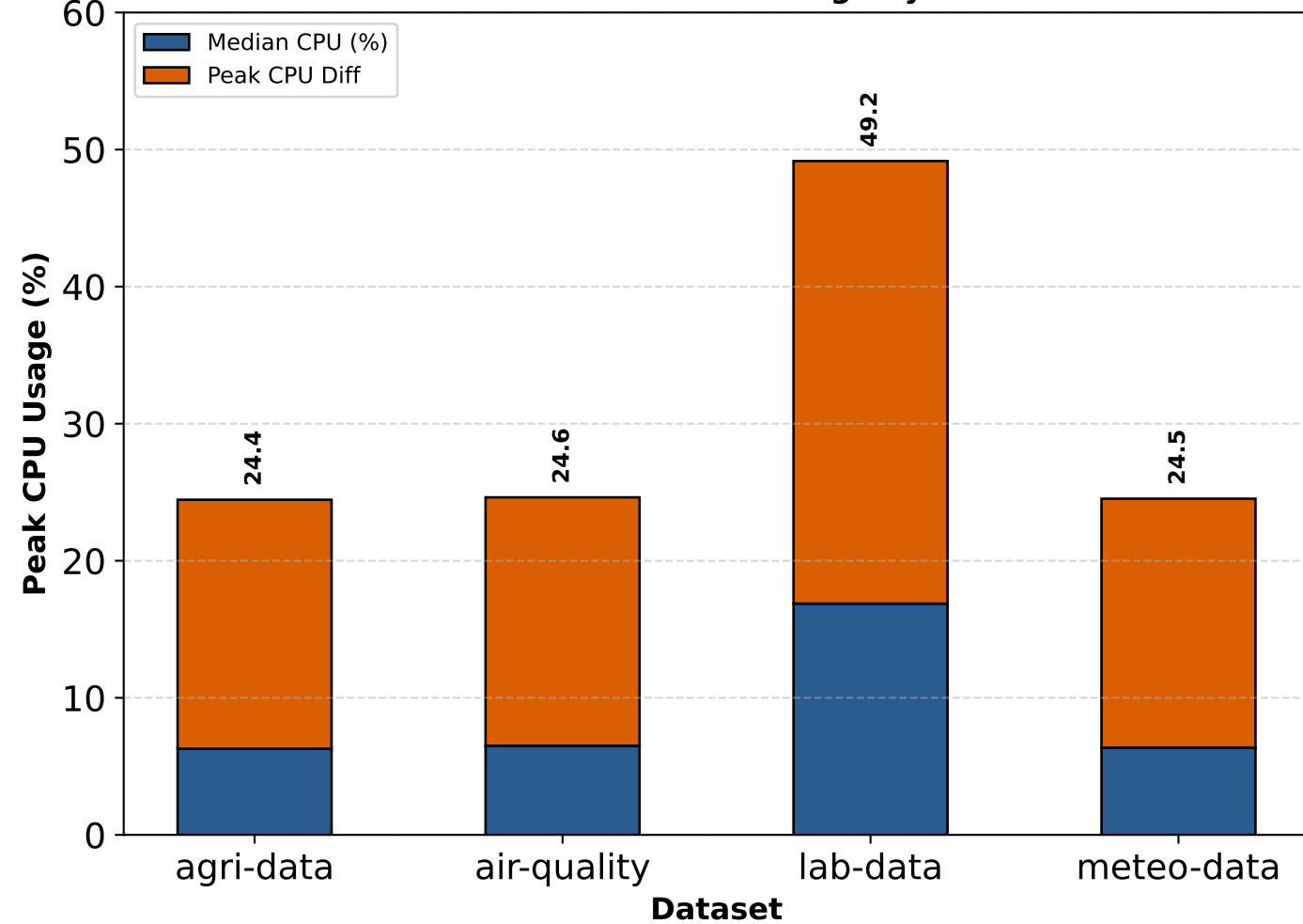
D. Median vs Peak CPU Usage by Dataset
