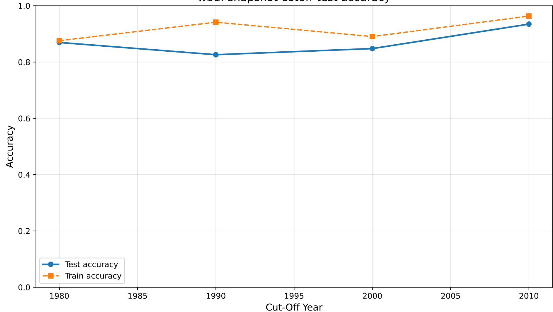
wbd: snapshot cutoff test accuracy
