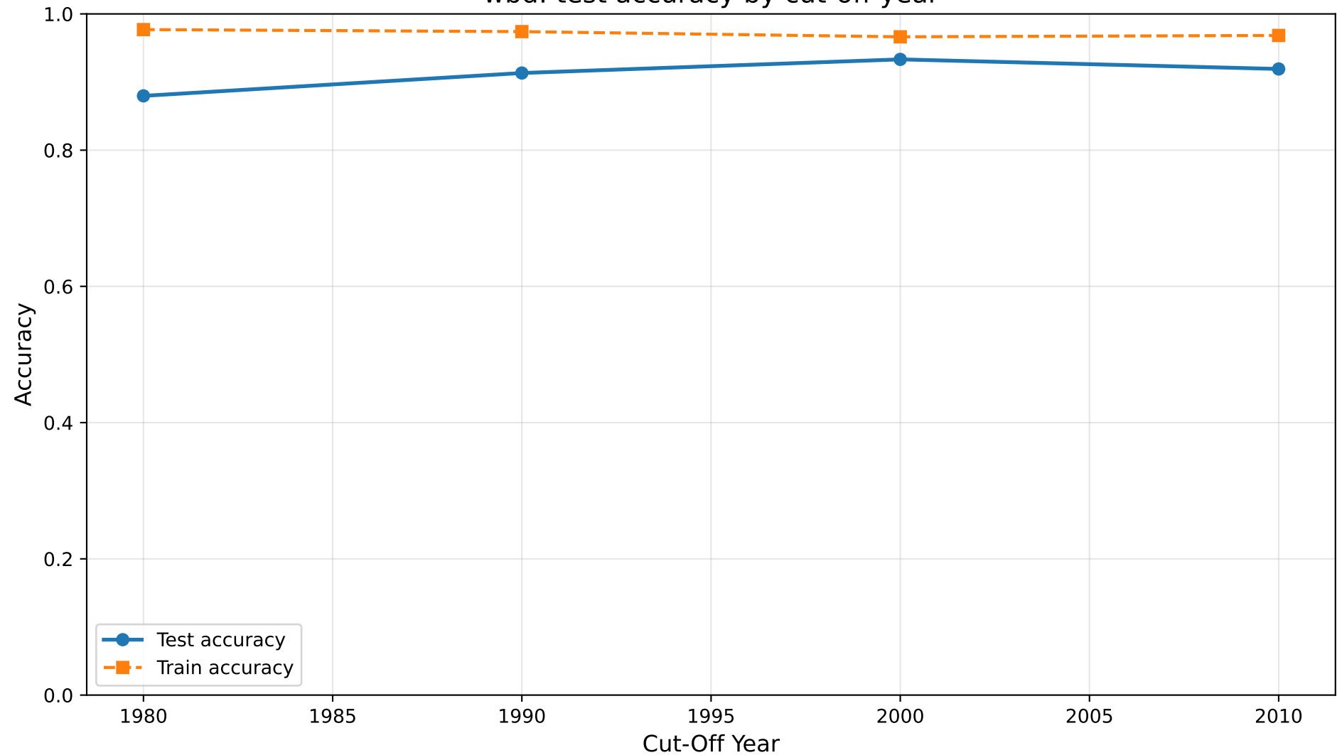
wbd: test accuracy by cut-off year
