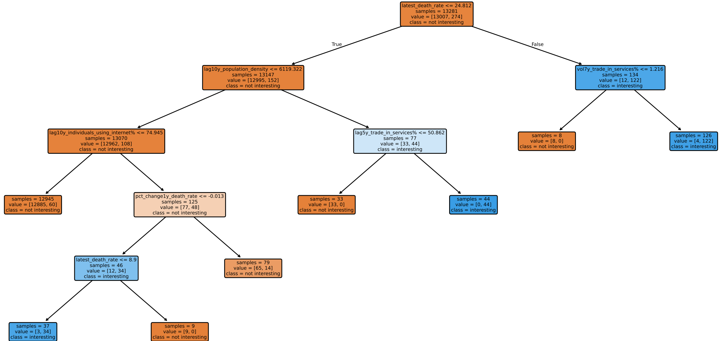
Tree 0 (acc=0.9916)
