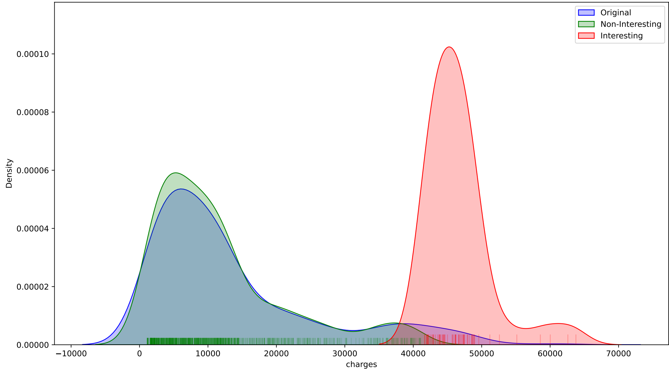
insurance: original target distribution
