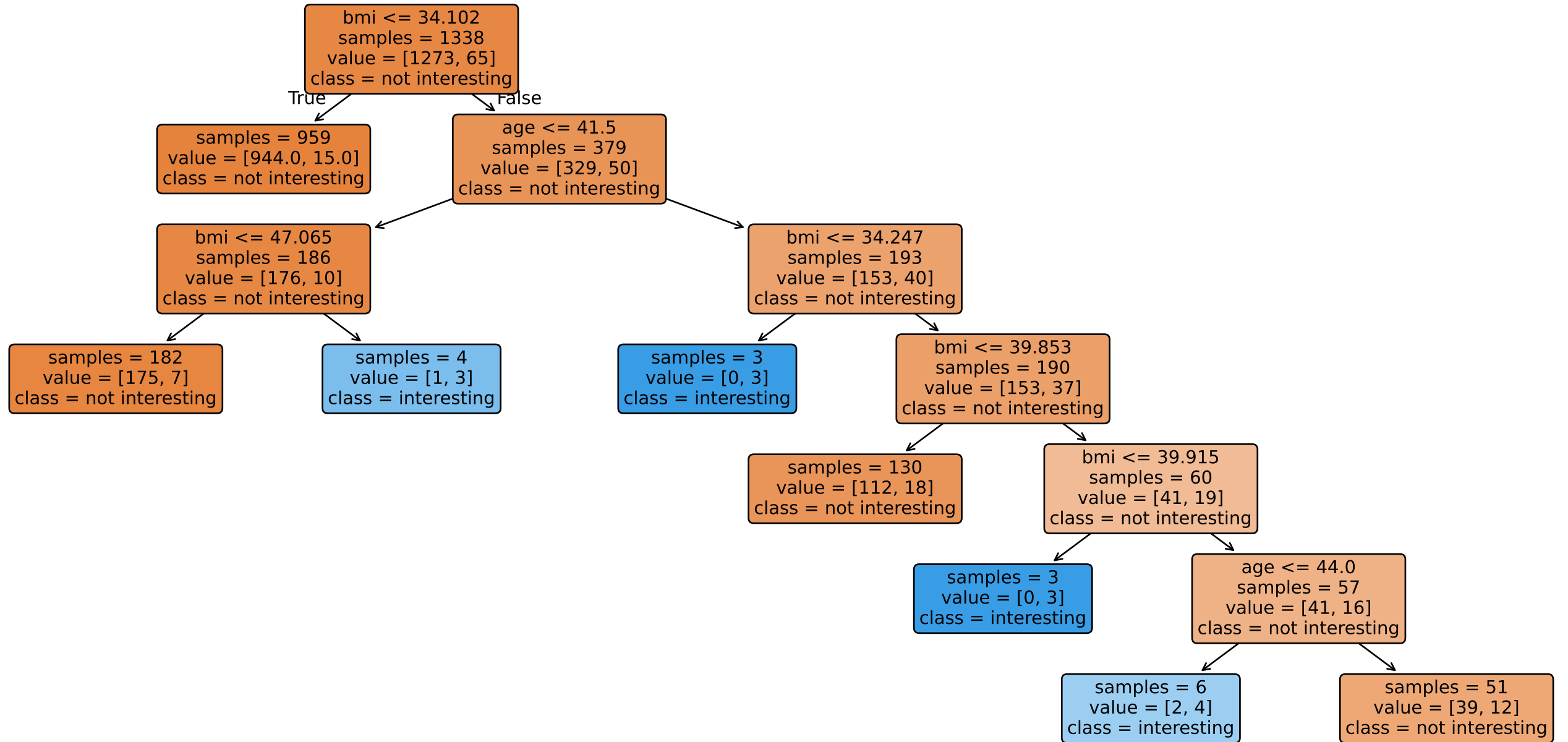
Tree 0 (acc=0.9537)
