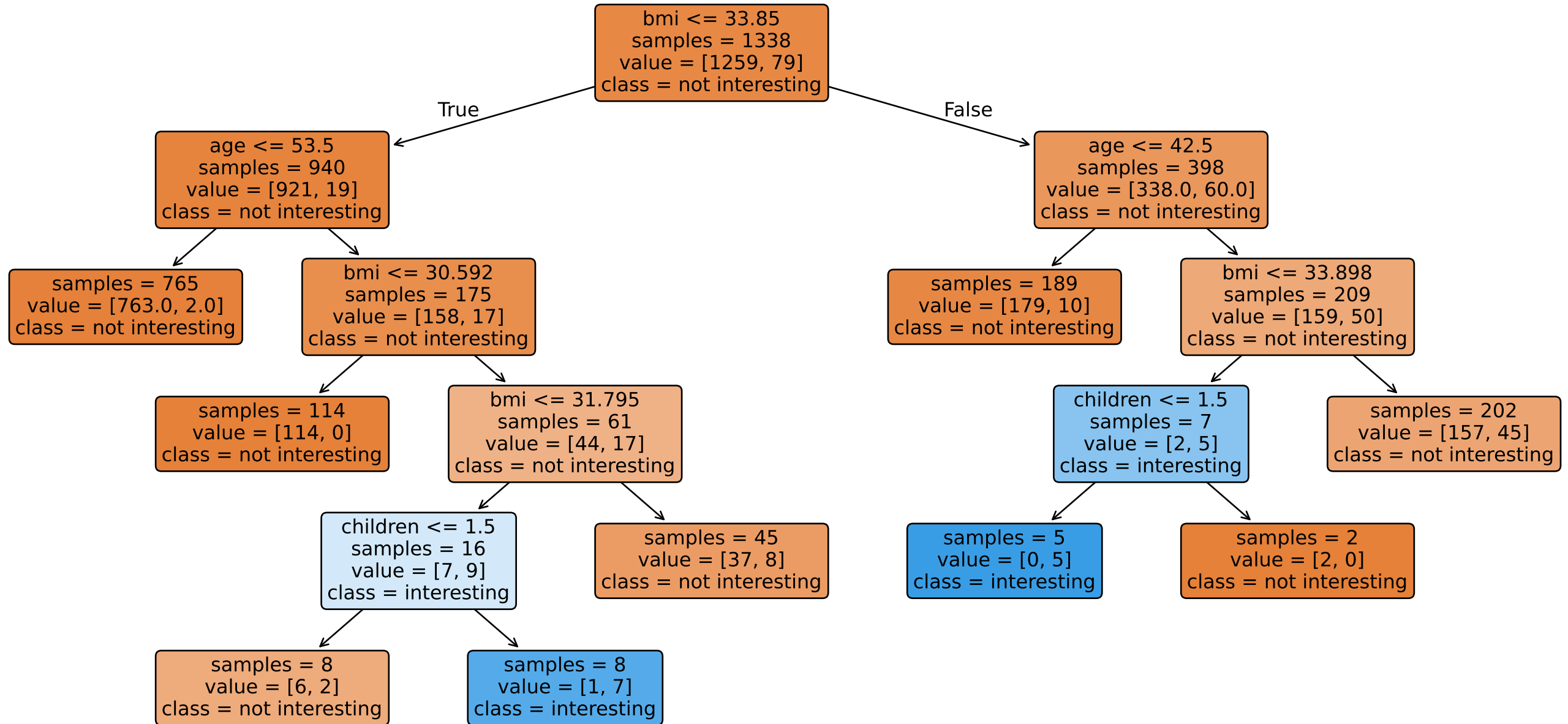
Tree 1 (acc=0.9522)
