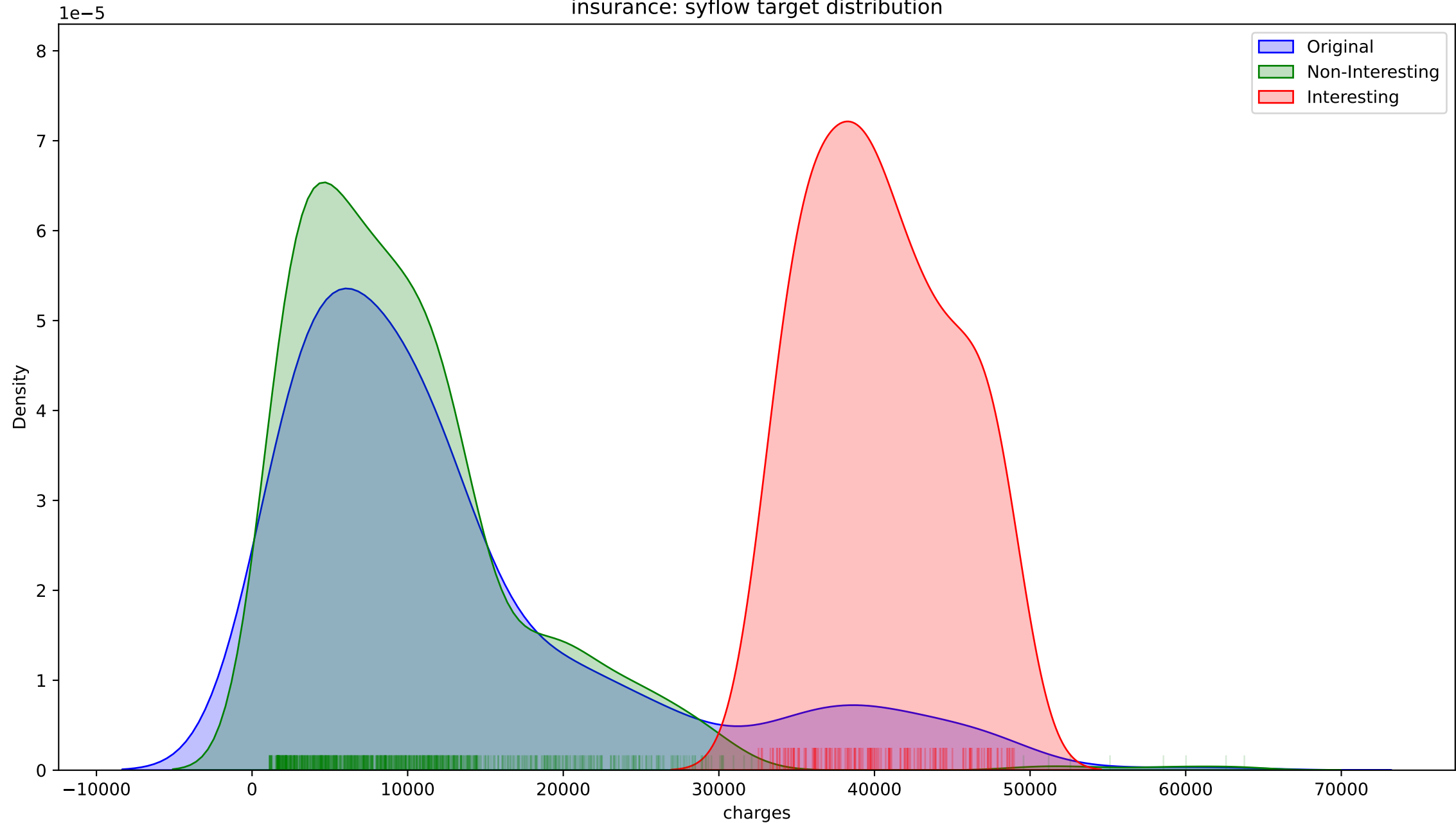
insurance: syflow target distribution
