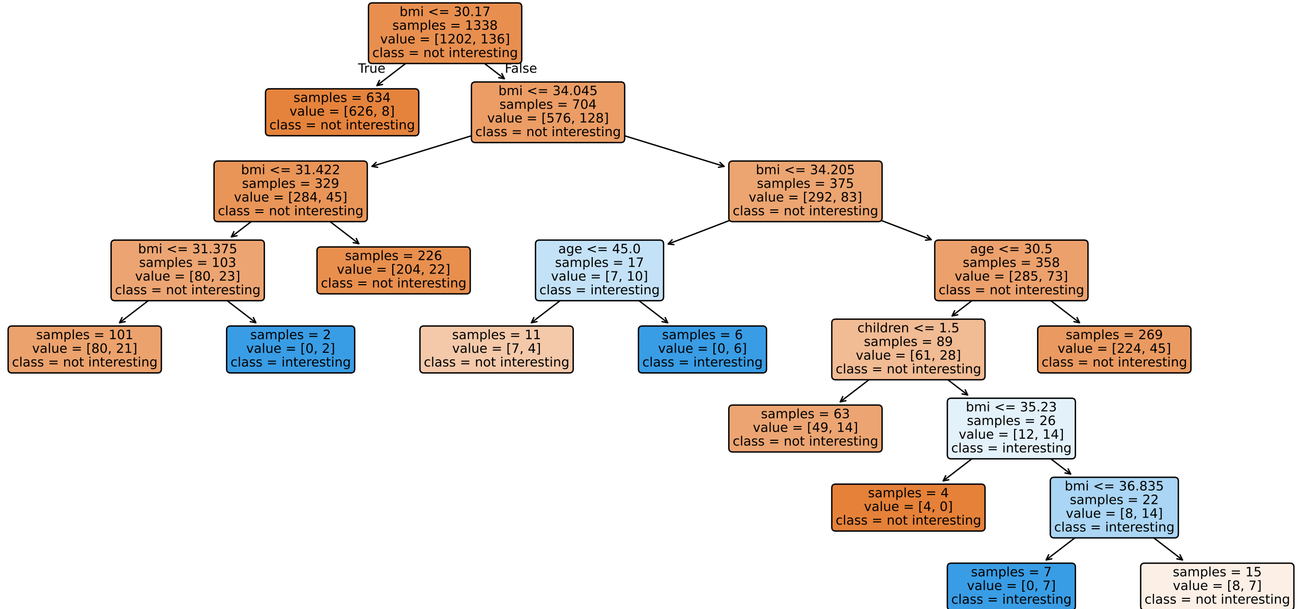
Tree 0 (acc=0.8931)
