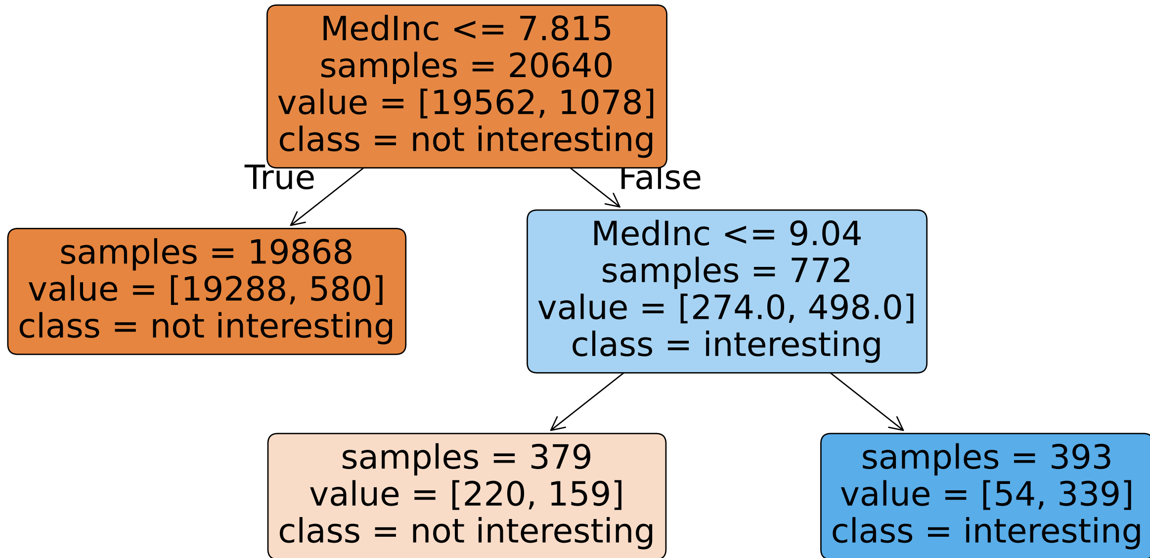
Tree 1 (acc=0.9624)
