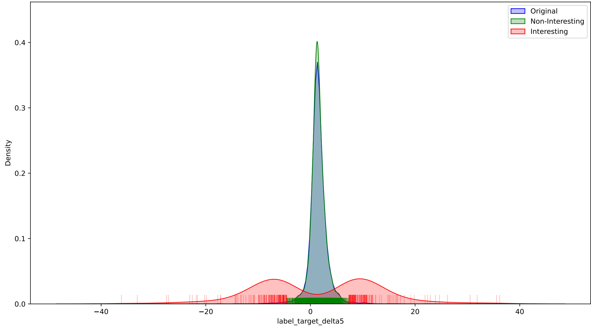
wbd_delta: tail_cluster target distribution
