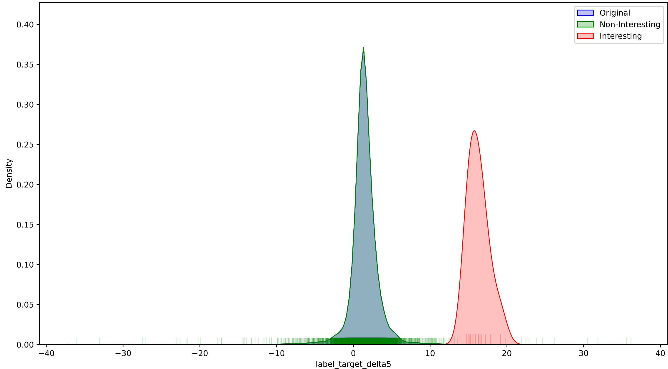
wbd_delta: timetribes target distribution
