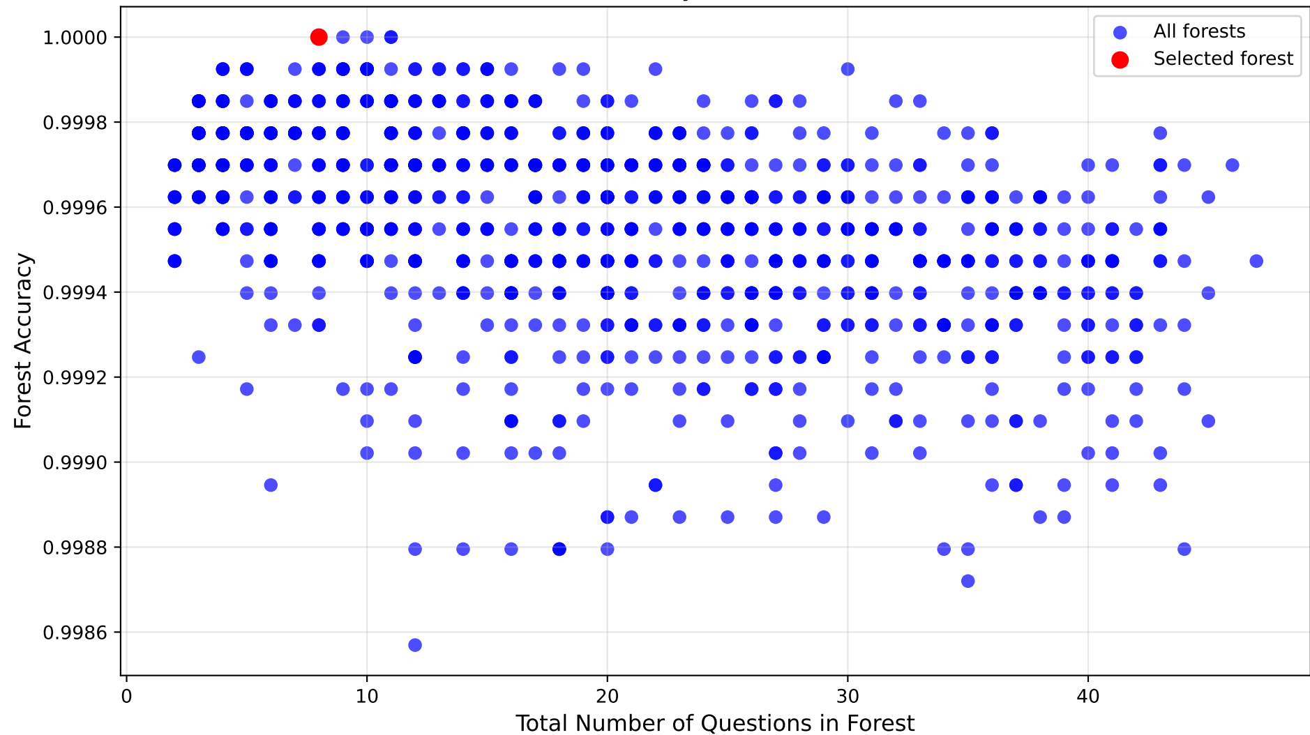
Forest Accuracy vs Total Questions
