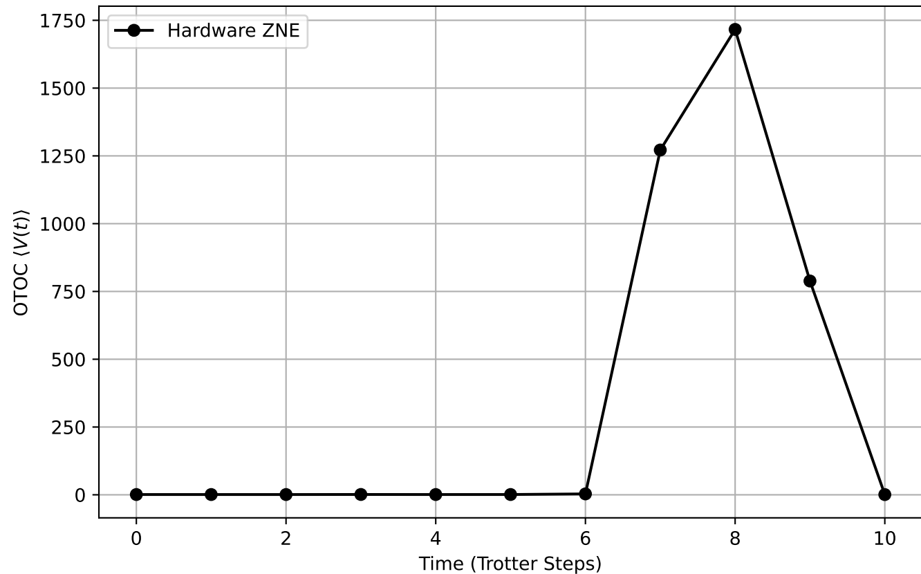
Hardware-Measured Information Scrambling ( \lambda_L = 1.2593 )
