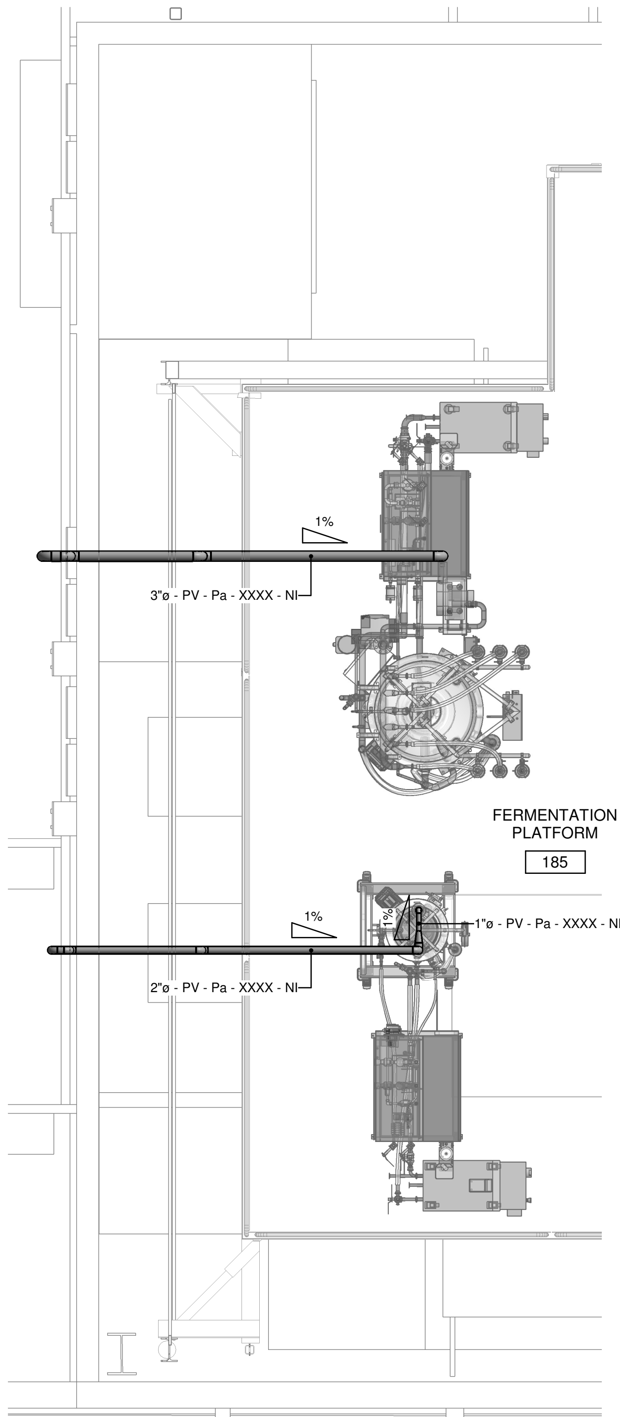
1 FERMENTATION - PROCESS VENT RUNOUT LAYOUT 3/8" = 1'-0"
