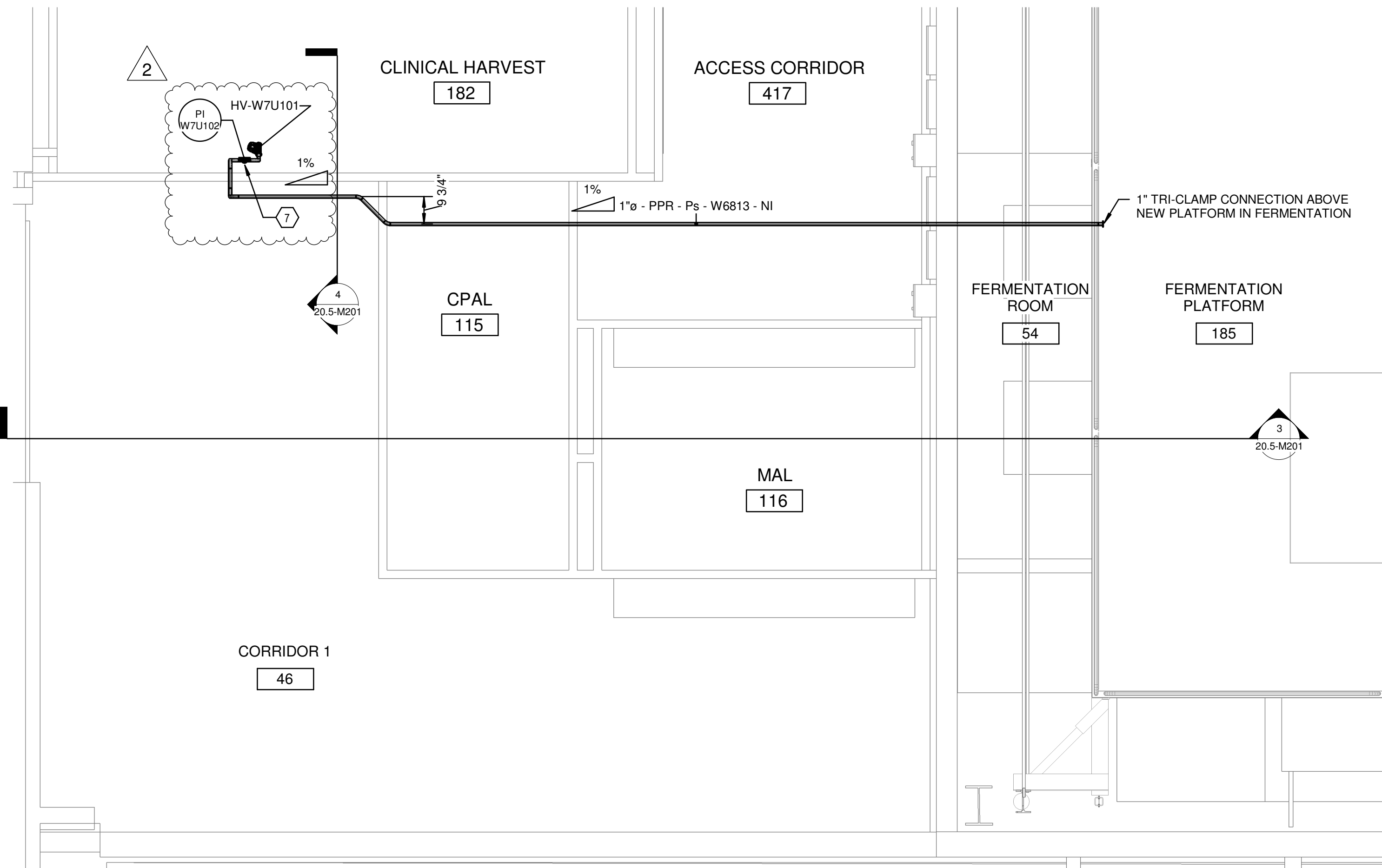
1 FERMENTATION - PROCESS PRODUCT LAYOUT 3/8" = 1'-0"
