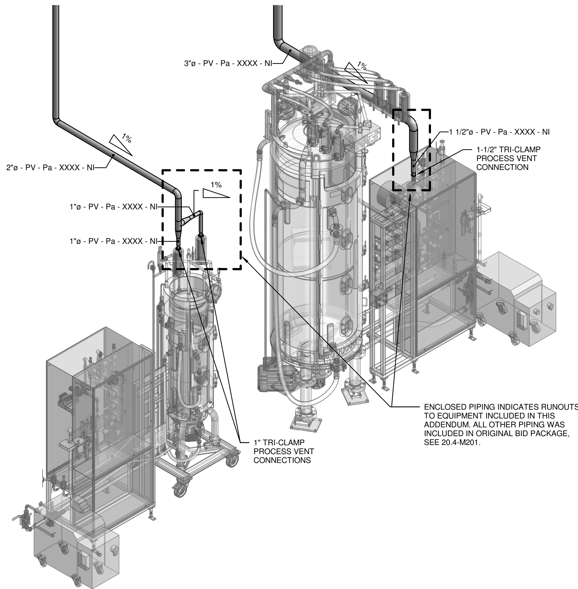
2 FERMENTATION - PROCESS VENT RUNOUT ISOMETRIC
