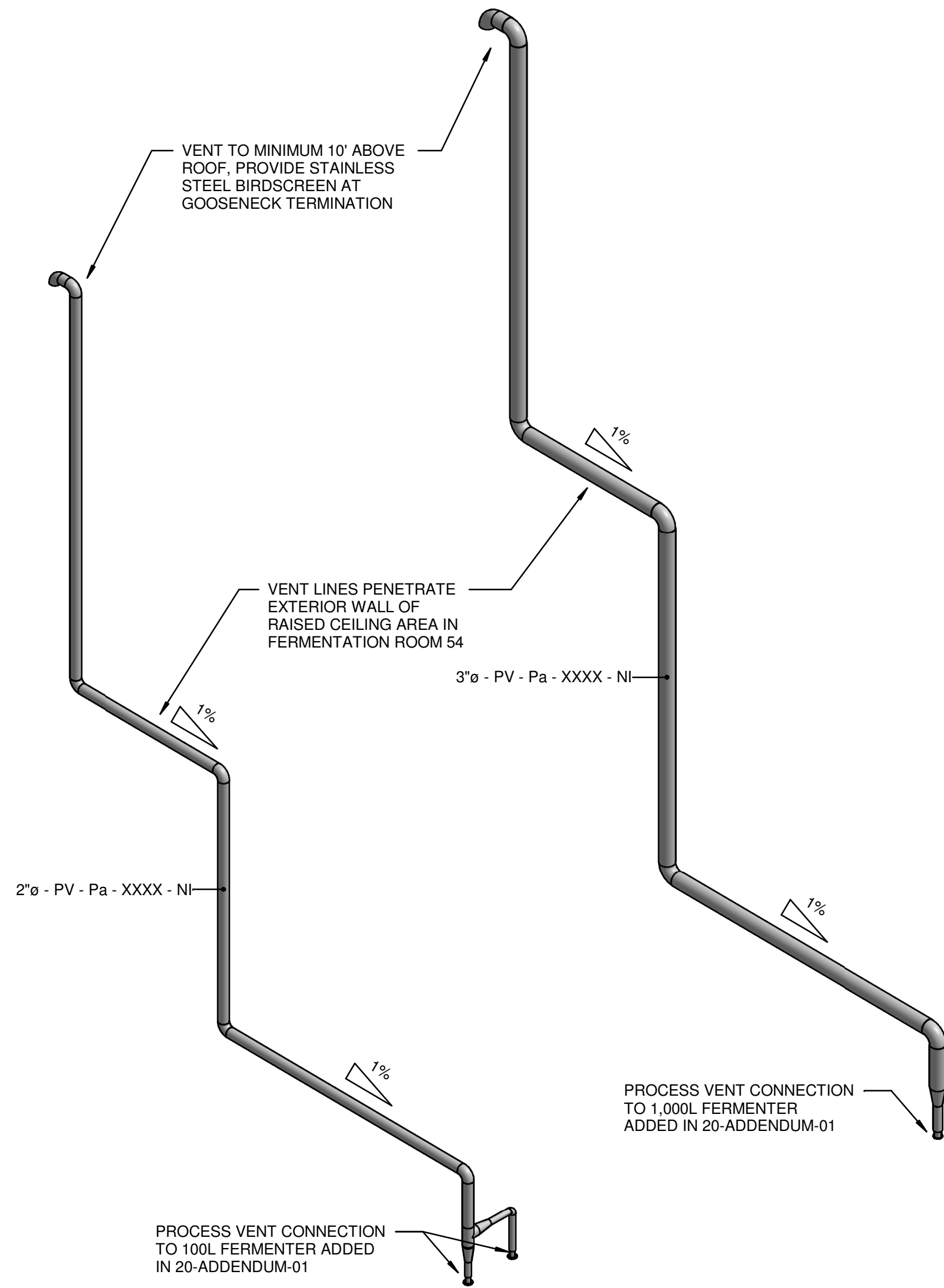
2 FERMENTATION - PROCESS VENT ISOMETRIC 3/8" = 1'-0"
