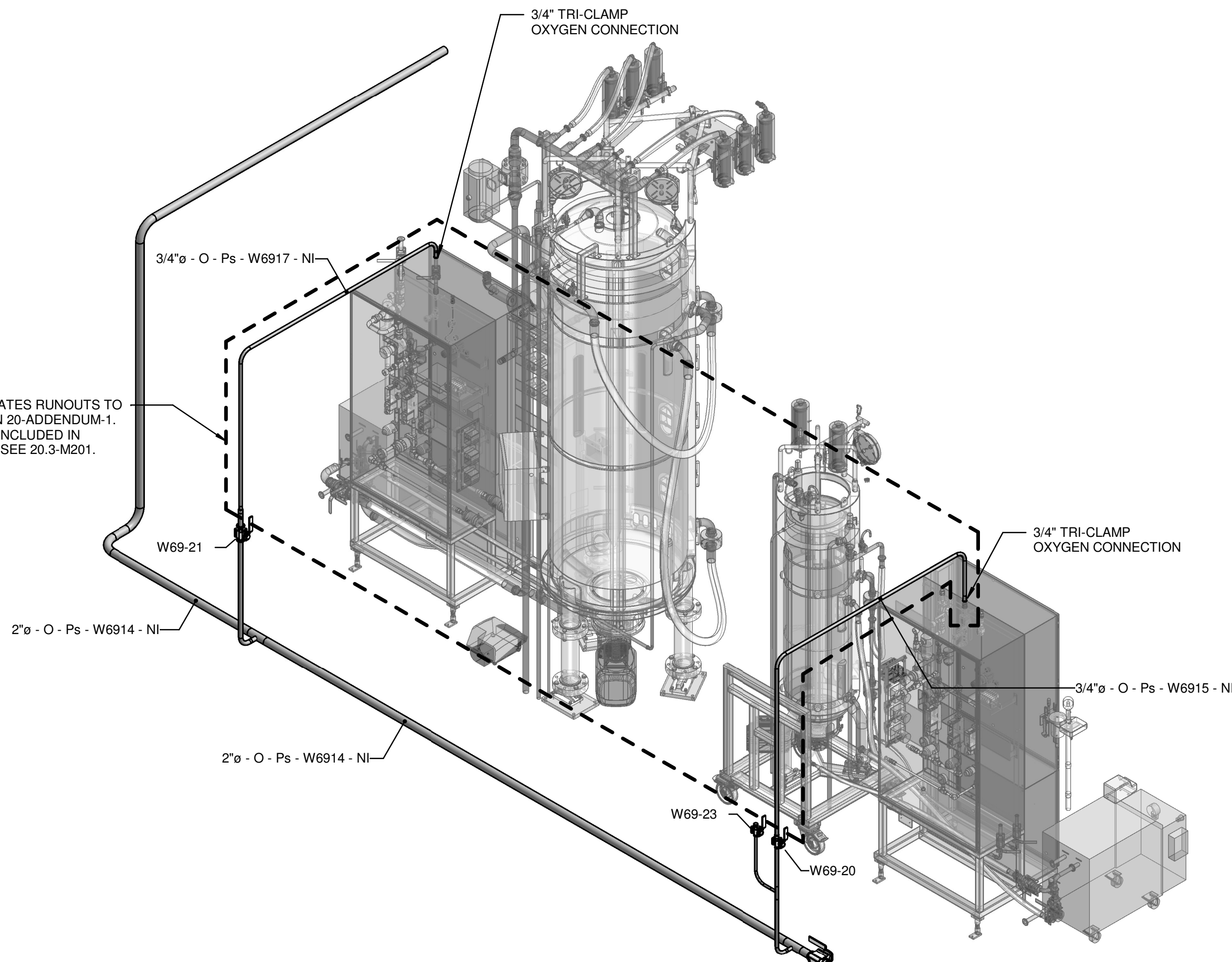
2 FERMENTATION - OXYGEN RUNOUTS ISOMETRIC
