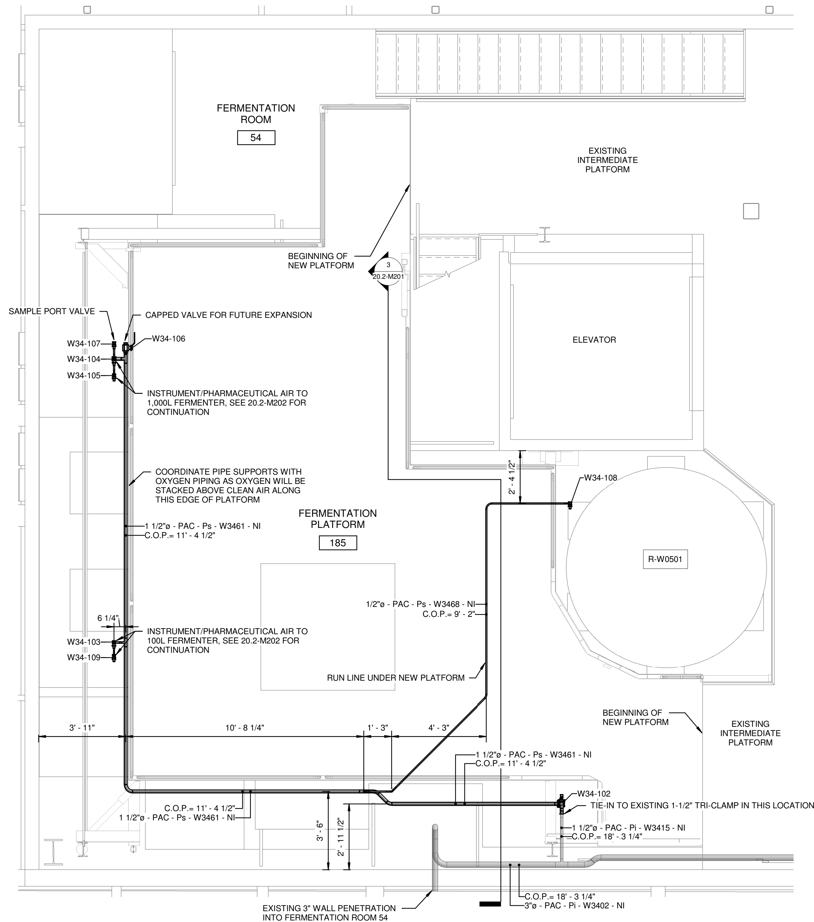
1 FERMENTATION - CLEAN AIR LAYOUT 3/8" = 1'-0"
