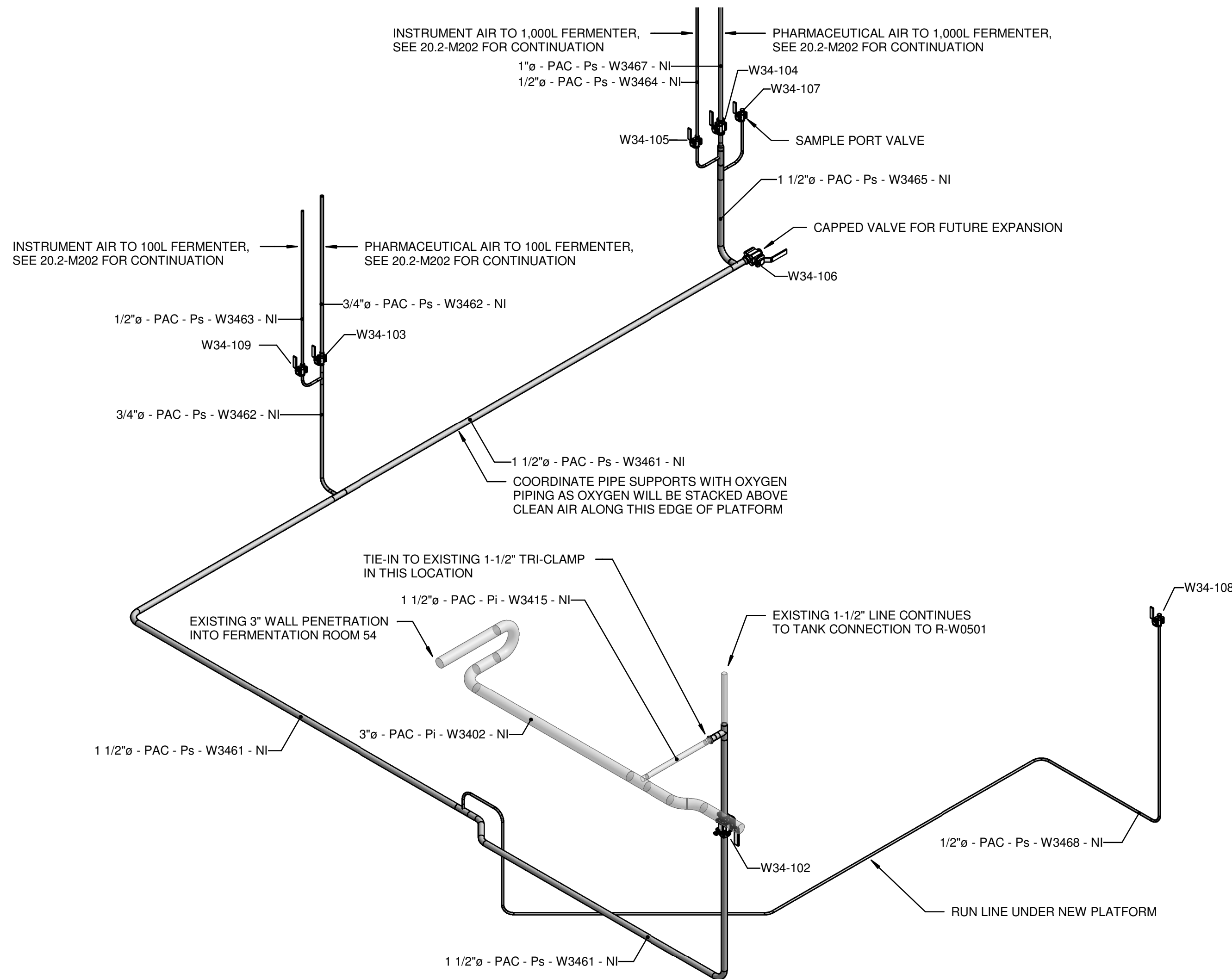
2 FERMENTATION - CLEAN AIR ISOMETRIC
