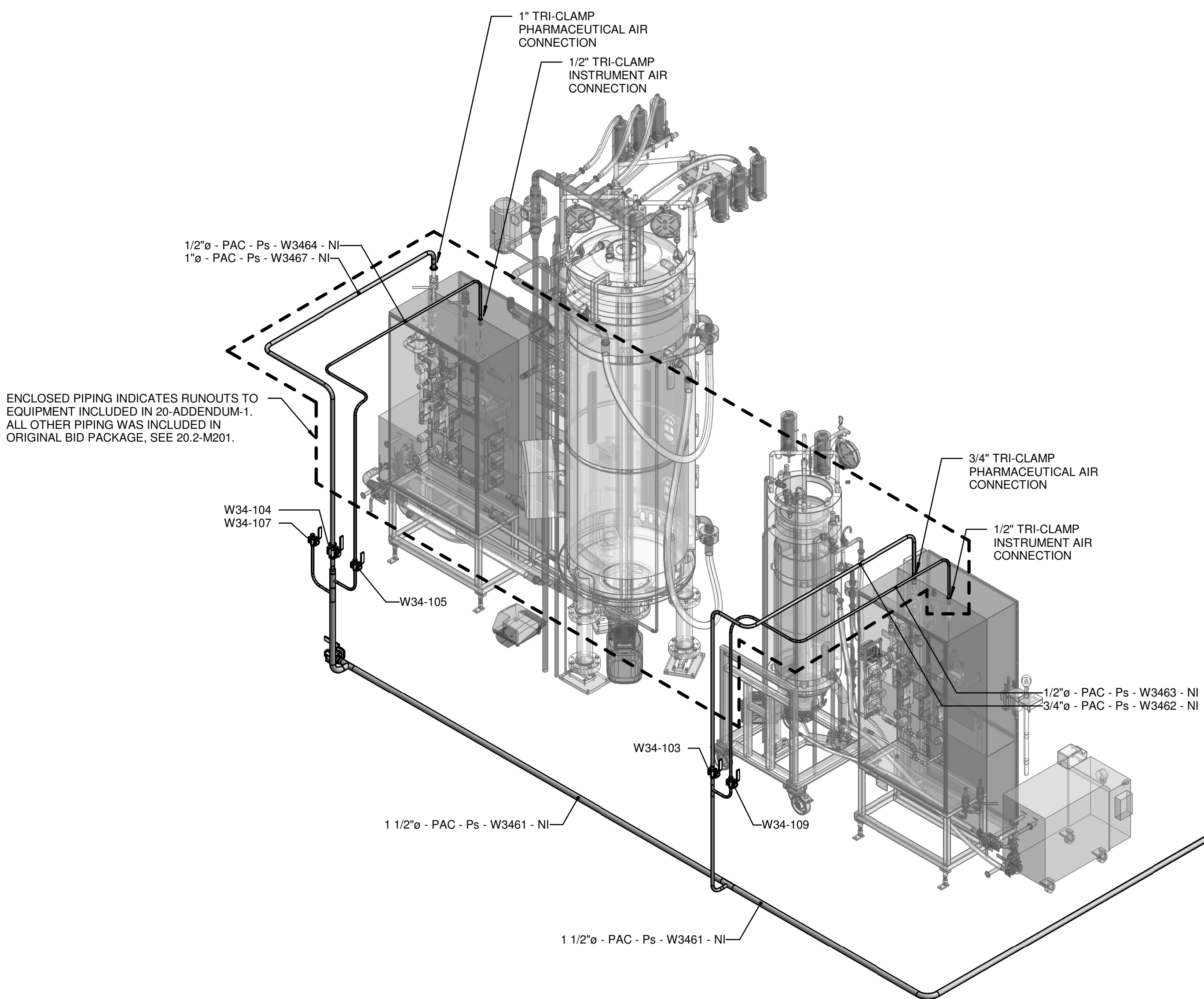
2 FERMENTATION - CLEAN AIR RUNOUTS ISOMETRIC
