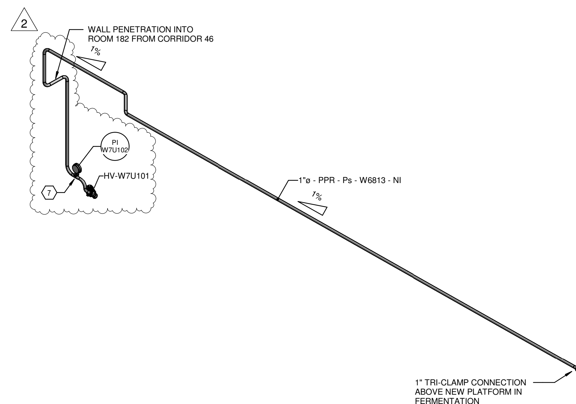
2 FERMENTATION - PROCESS PRODUCT ISOMETRIC
