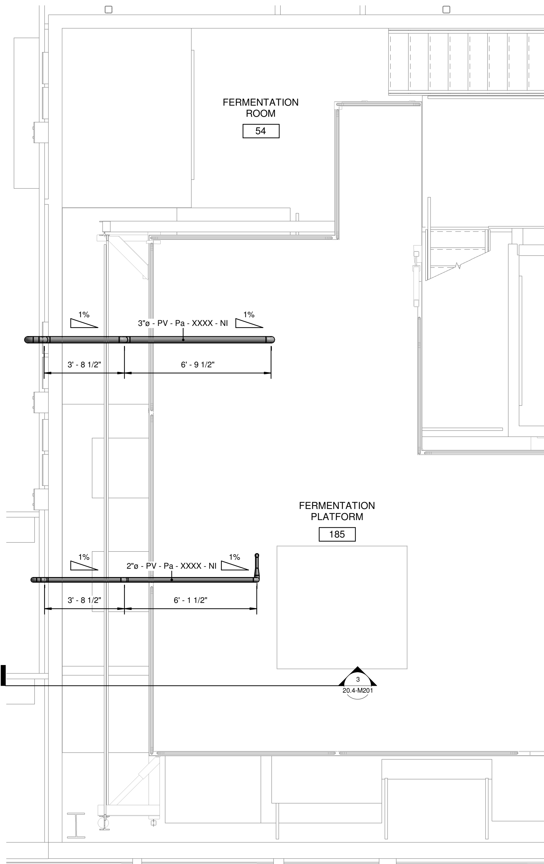
1 FERMENTATION - PROCESS VENT LAYOUT 3/8" = 1'-0"
