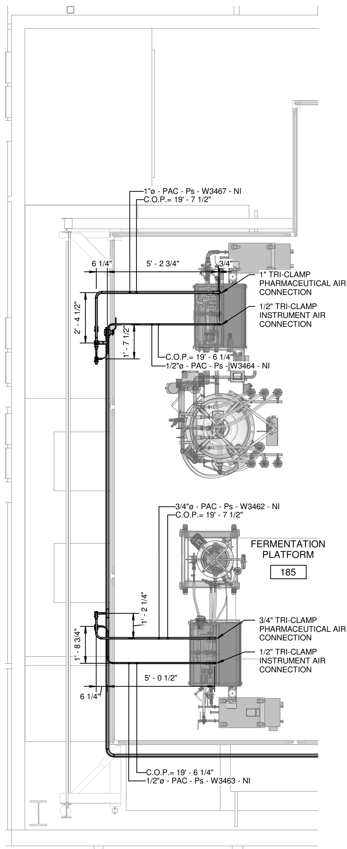
1 FERMENTATION - CLEAN AIR RUNOUTS LAYOUT 3/8" = 1'-0"
