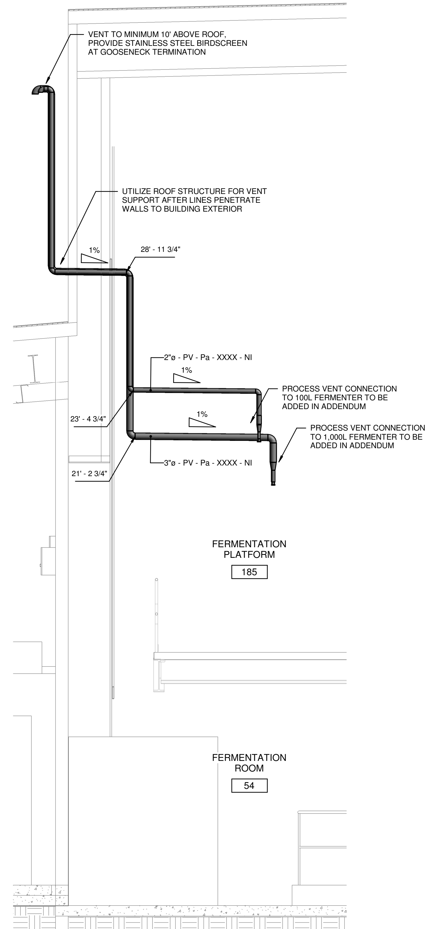
3 FERMENTATION - PROCESS VENT SECTION 3/8" = 1'-0"
