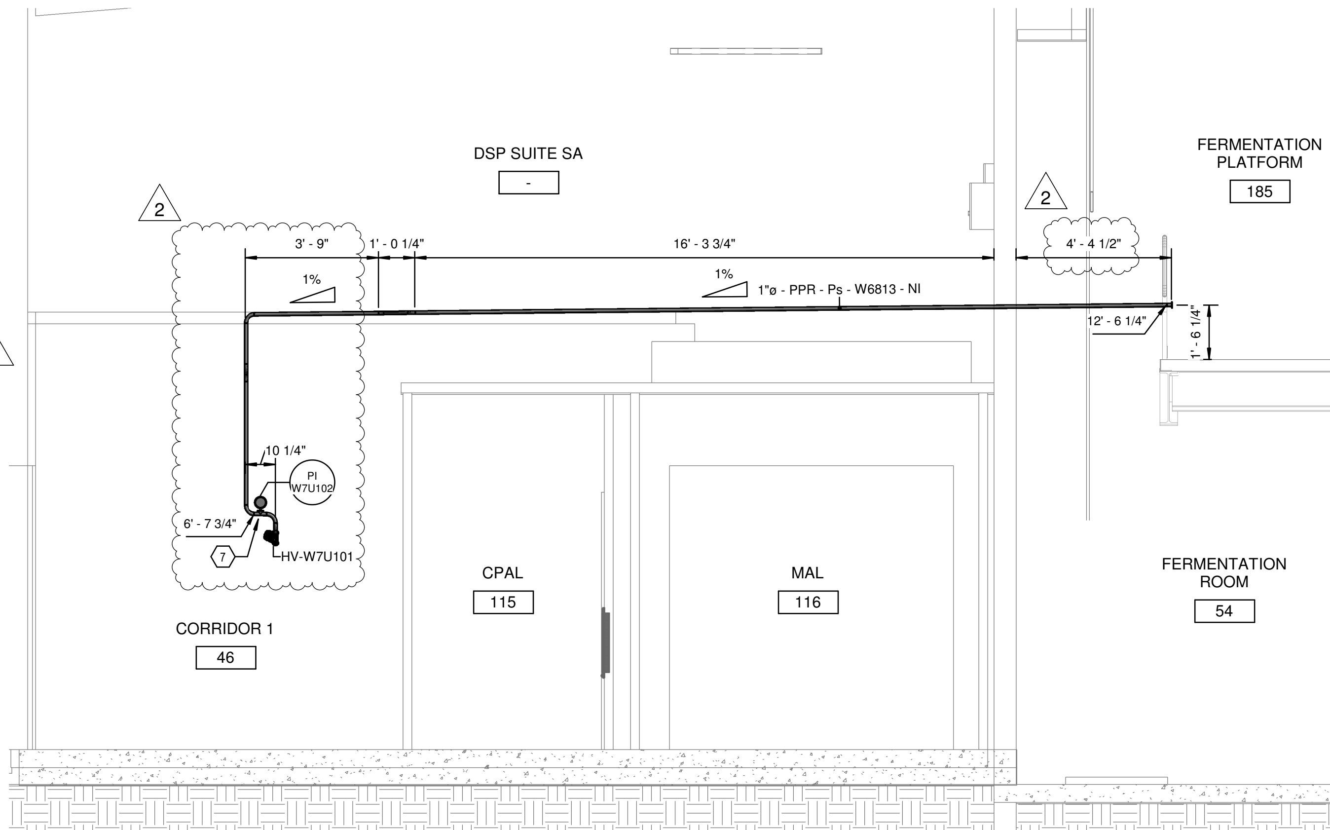
3 FERMENTATION - PROCESS PRODUCT SECTION 1 3/8" = 1'-0"
