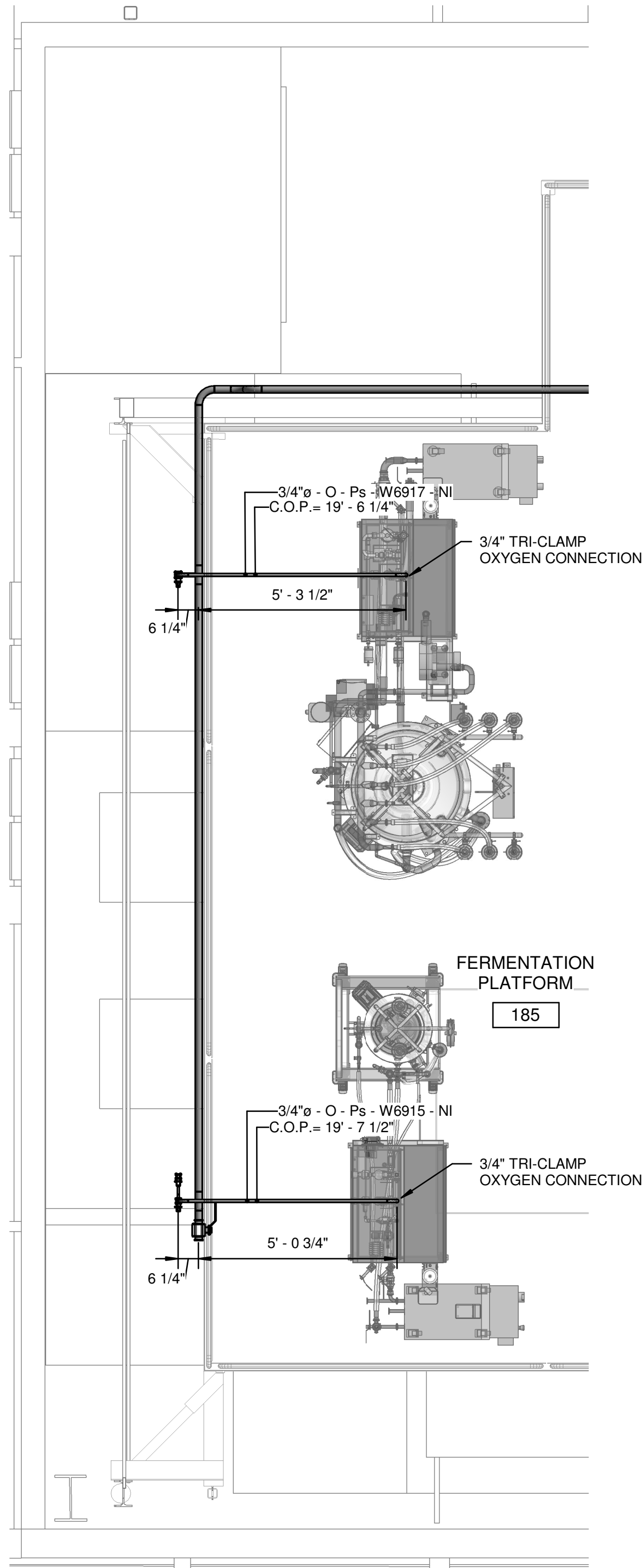
1 FERMENTATION - OXYGEN RUNOUTS LAYOUT 3/8" = 1'-0"
