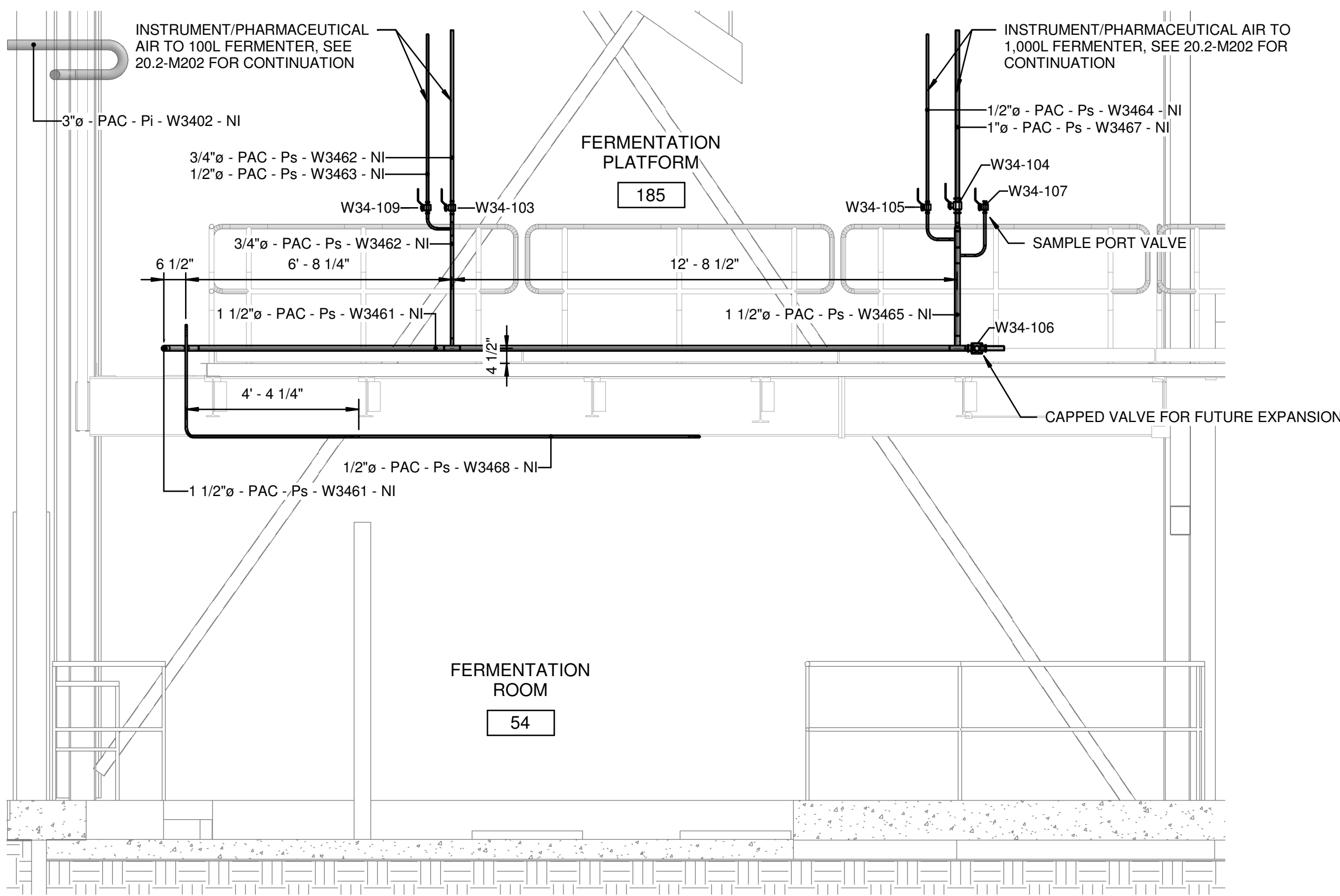
3 FERMENTATION - CLEAN AIR SECTION 3/8" = 1'-0"
