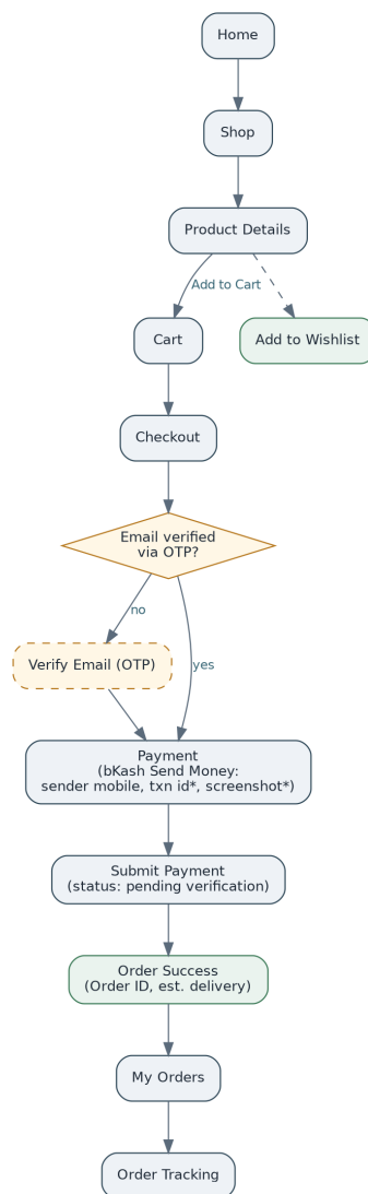
Fig 5. Customer purchase flow with OTP and manual-bKash branch.
