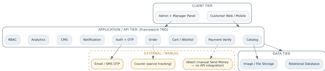
Fig 6. Reference architecture. Final framework pending your stack decision ($11C).
