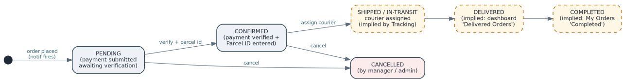
Fig 4. Order lifecycle. Solid = explicit in source; dashed = implied by other screens.
