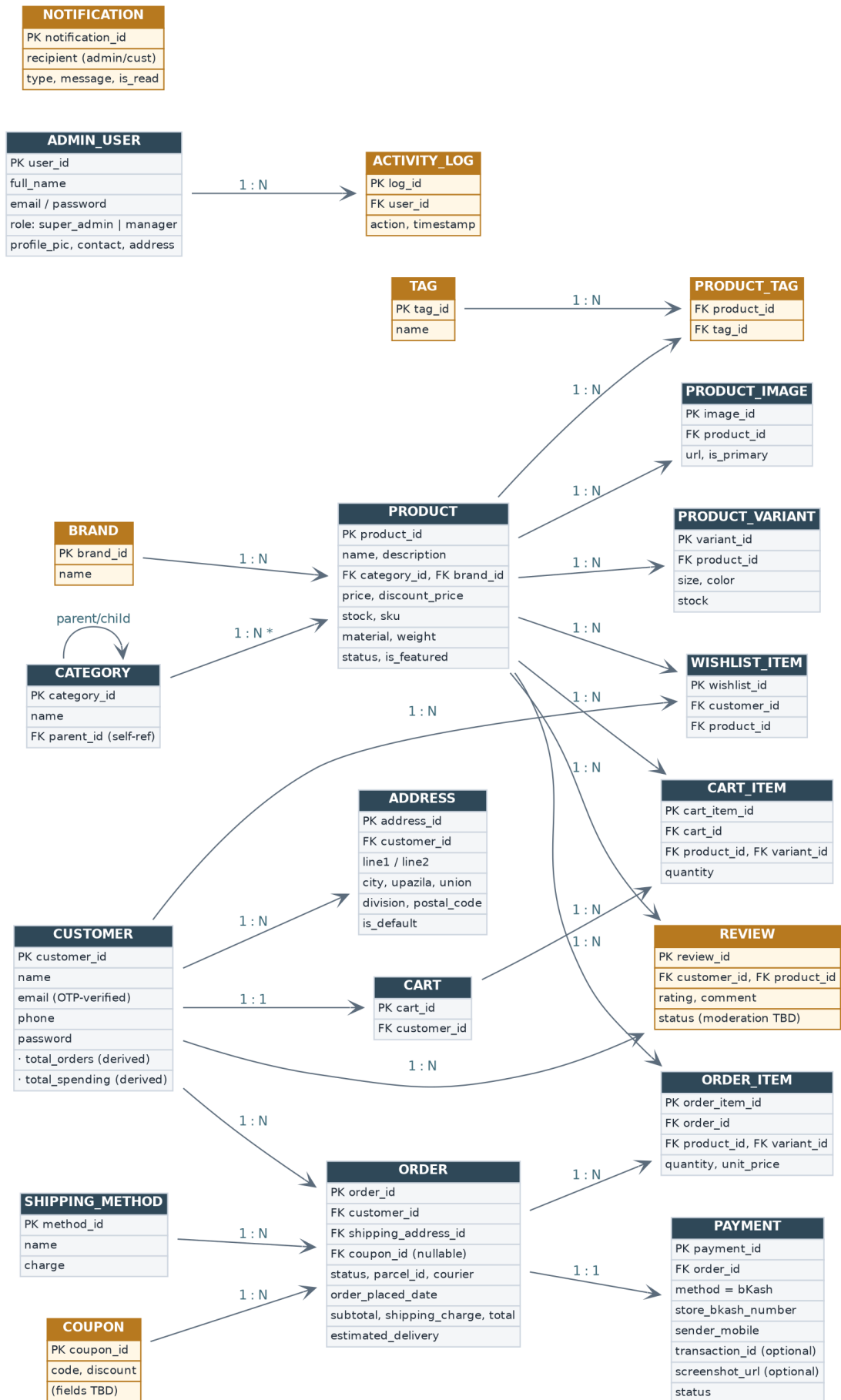
Fig 3. Entity relationship model (inferred). Amber = provisional / undefined module.
