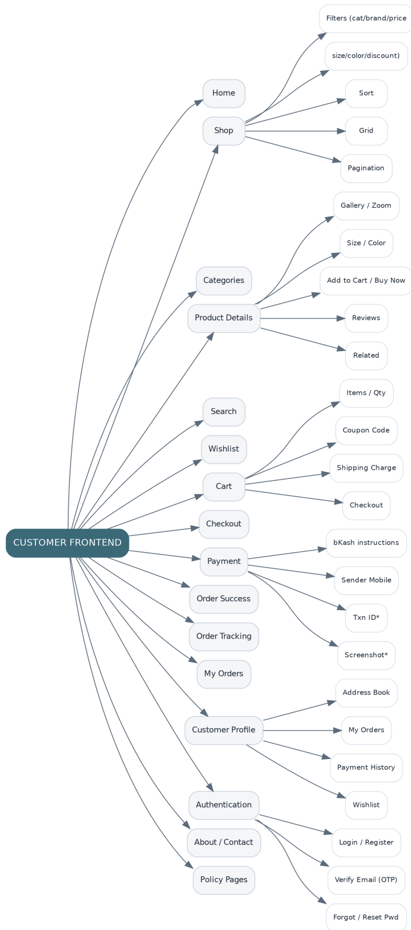
Fig 2. Customer storefront module map.
