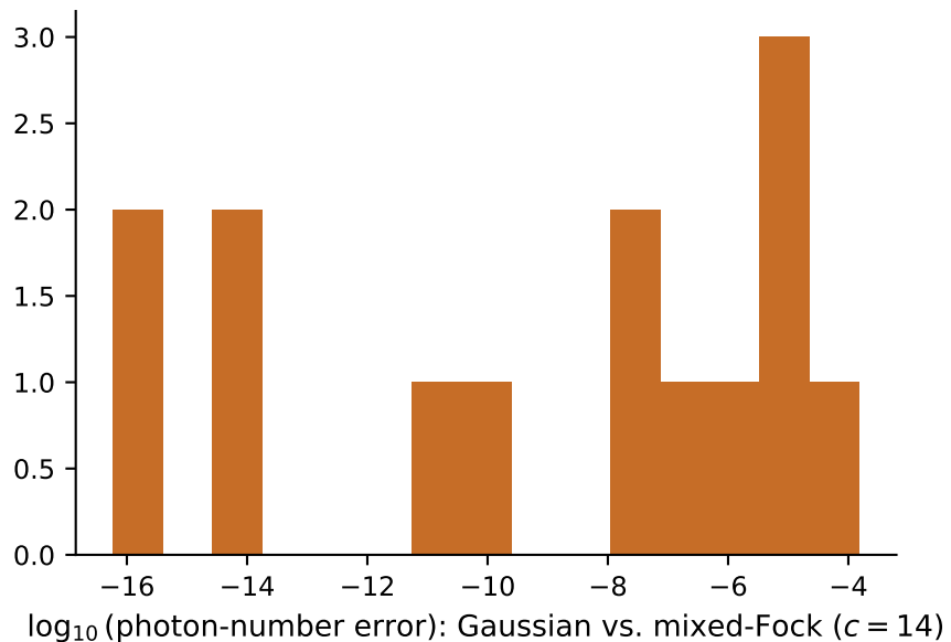
Backend cross-checks: exact (left) vs. finite-cutoff approximation (right)
