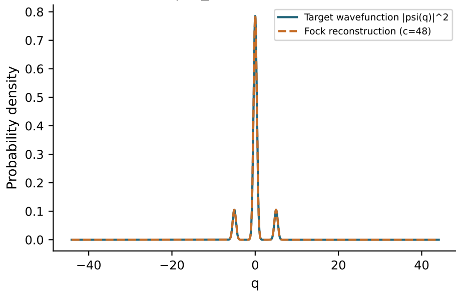
GKP |0\rangle_L , default (width=0.4)
