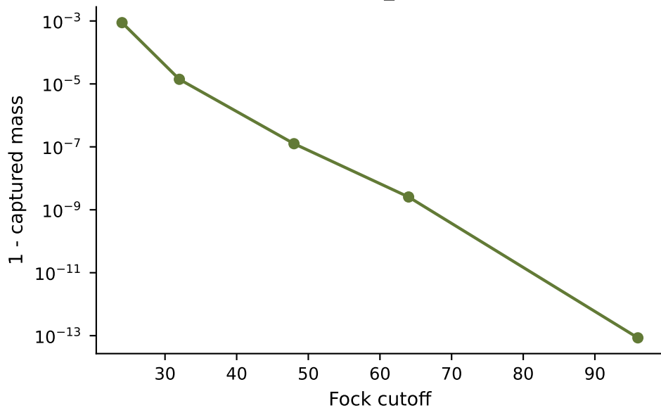
Cutoff sensitivity, peak_width=envelope=0.4
