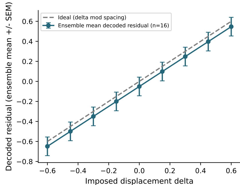
GKP q-syndrome extraction, finite ancilla (cutoff=80, width=0.35)
