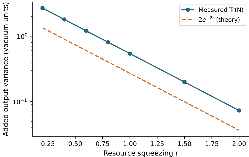
Four-step identity wire: finite-squeezing noise
