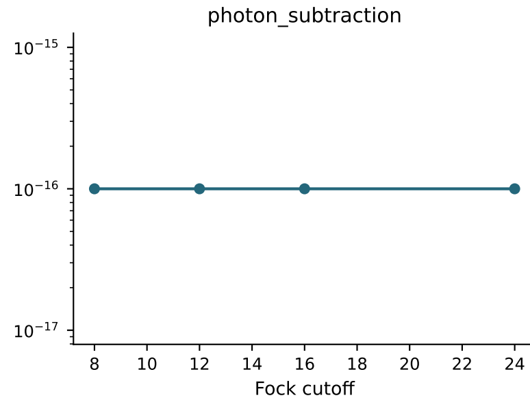
Fock cutoff convergence (highest cutoff is a reference, not exact truth)
