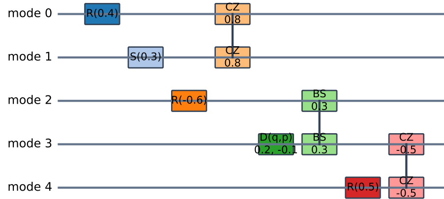
Photonic circuit
