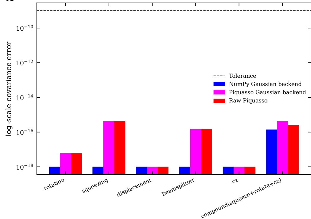
Covariance error vs. NumPy analytic target
