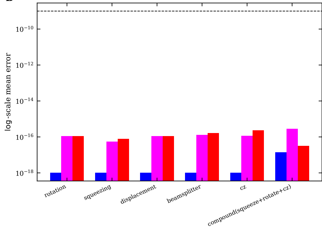
Mean error vs. NumPy analytic target
