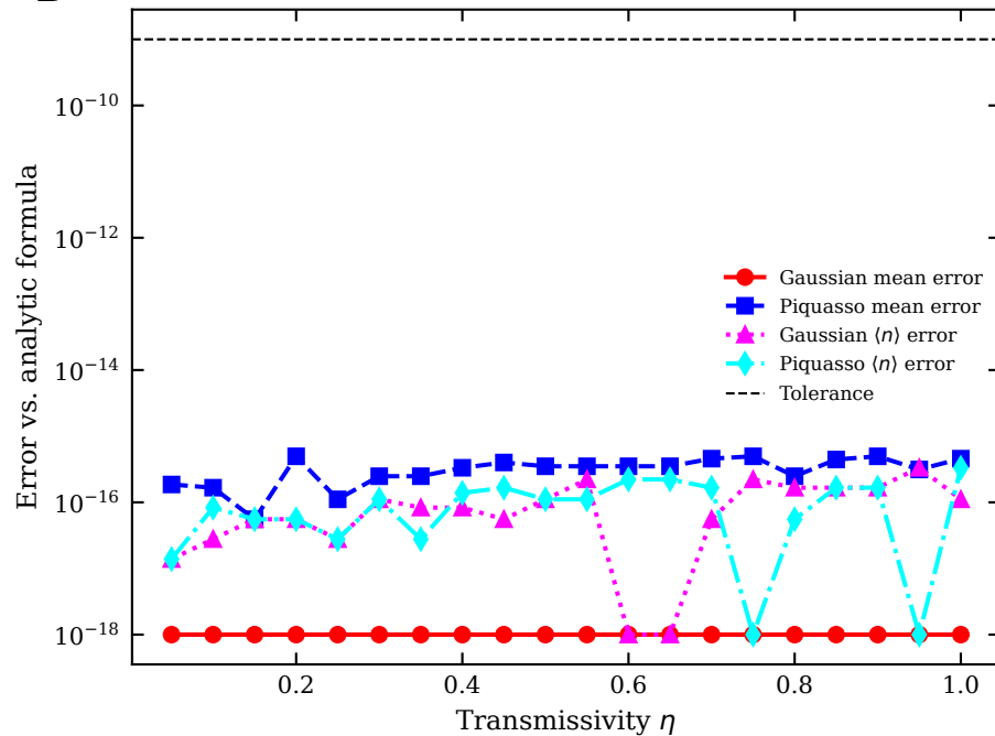
Exact-identity validation
