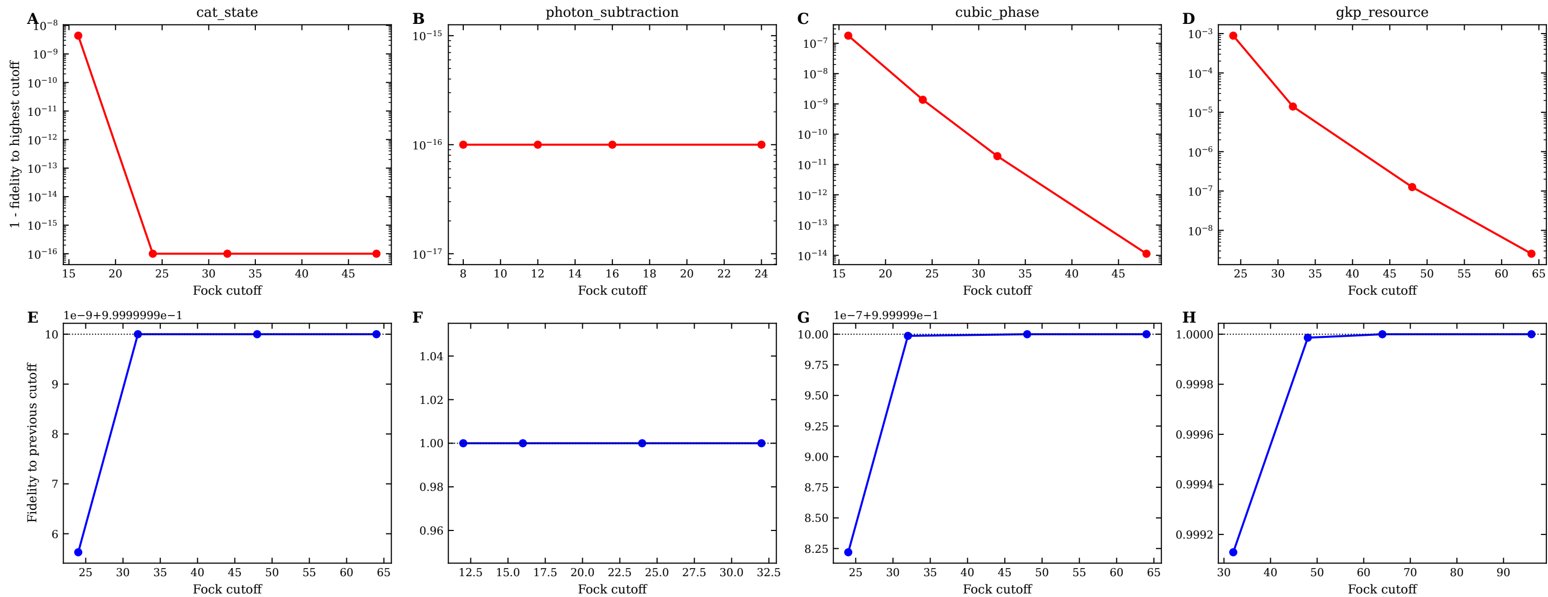
Fock cutoff convergence (top: vs. highest tested cutoff; bottom: successive refinements)
