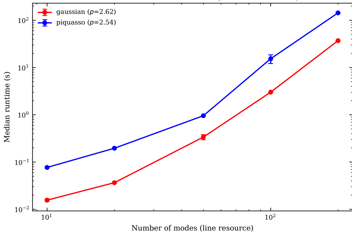
Gaussian backend runtime scaling (this machine only)
