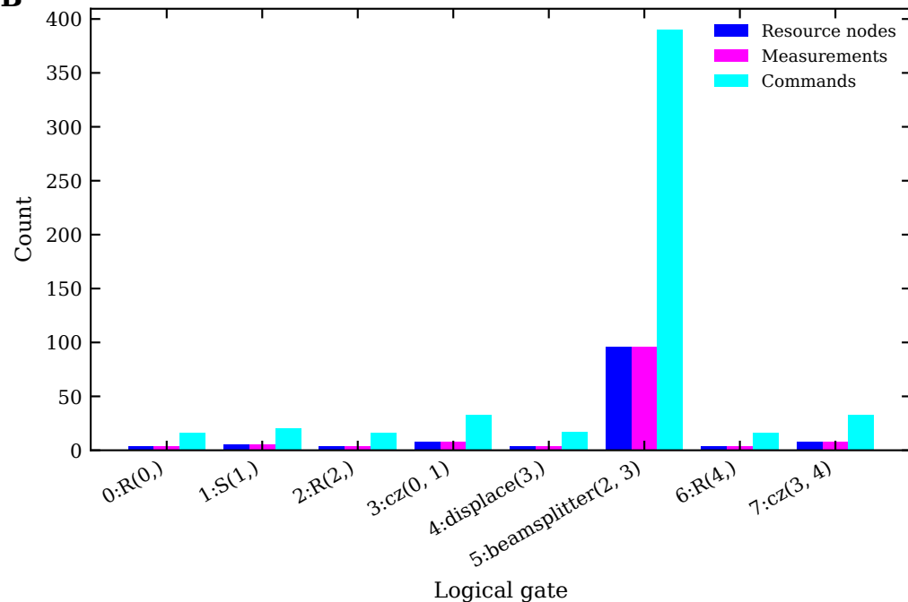
Per-gate provenance counts
