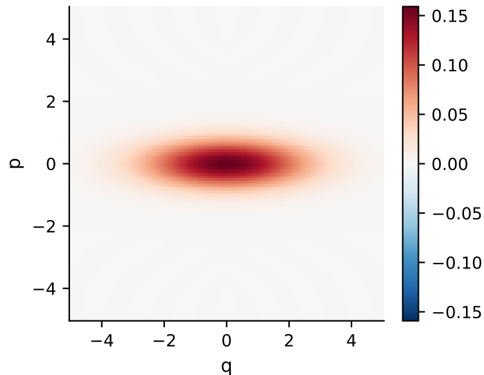
Before (squeezed vacuum)
