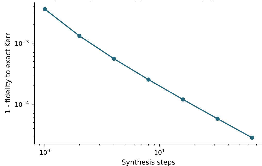
Kerr Lie-product synthesis, kappa=0.05 (direct physical execution)
