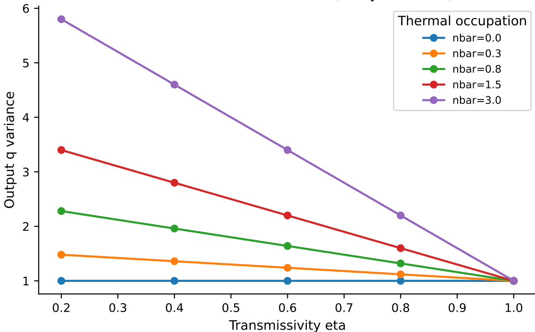
Thermal attenuation channel (analytic curves)
