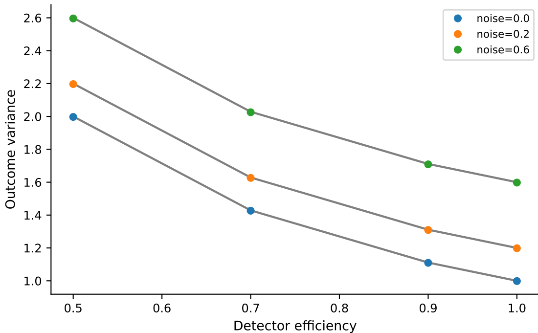
Noisy homodyne: sampled vs. documented formula (lines=analytic)
